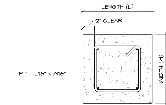
10 Pier Reinforcing Detail 1 1/2" = 1'-0"
