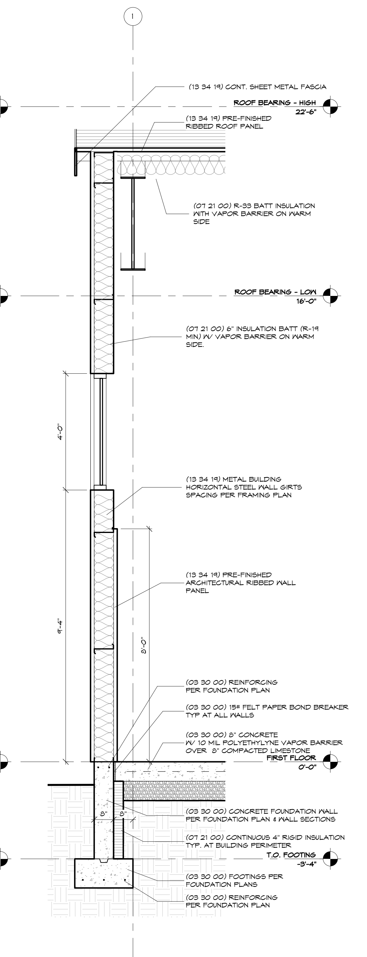
5 Wall Section 1/2" = 1'-0"
