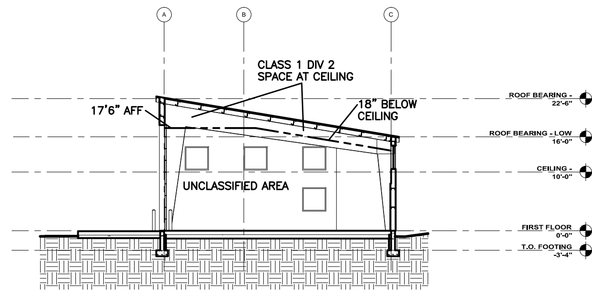
2 CNG CLASSIFIED CEILING SPACE 1/16" = 1'
