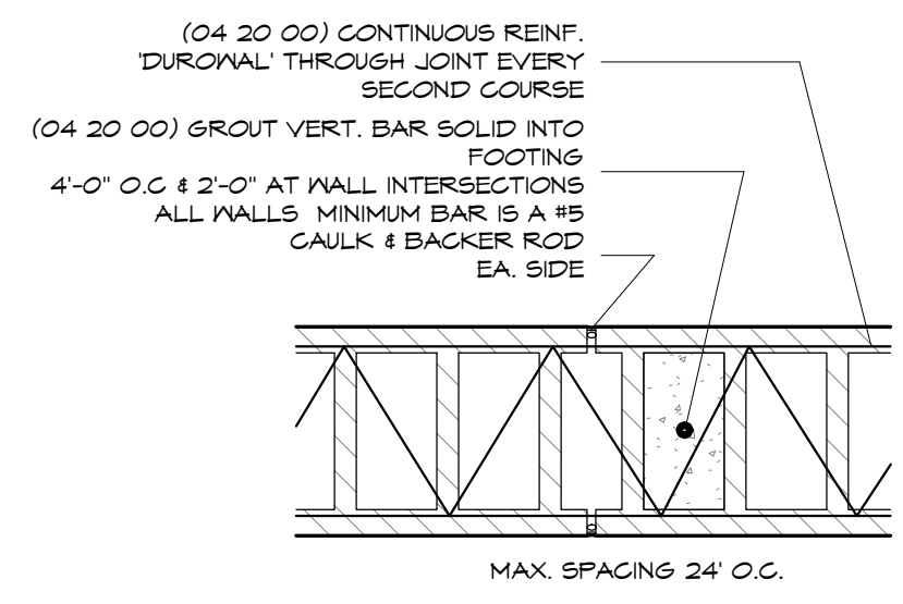
3 Masonry Control Joint 1 1/2" = 1'-0"
