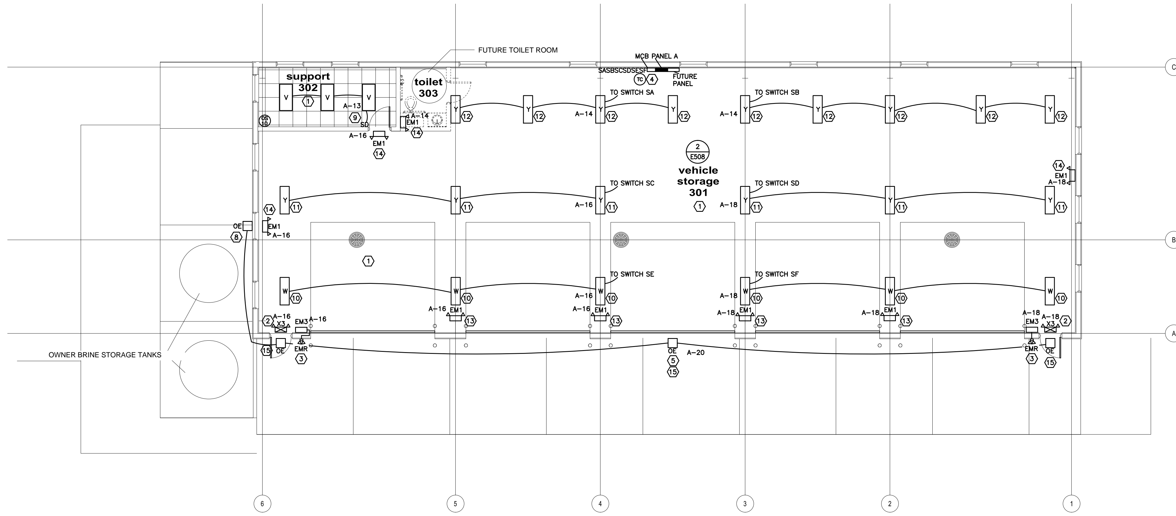
1 Satellite Building Lighting Plan 1/8" = 1'-0"
