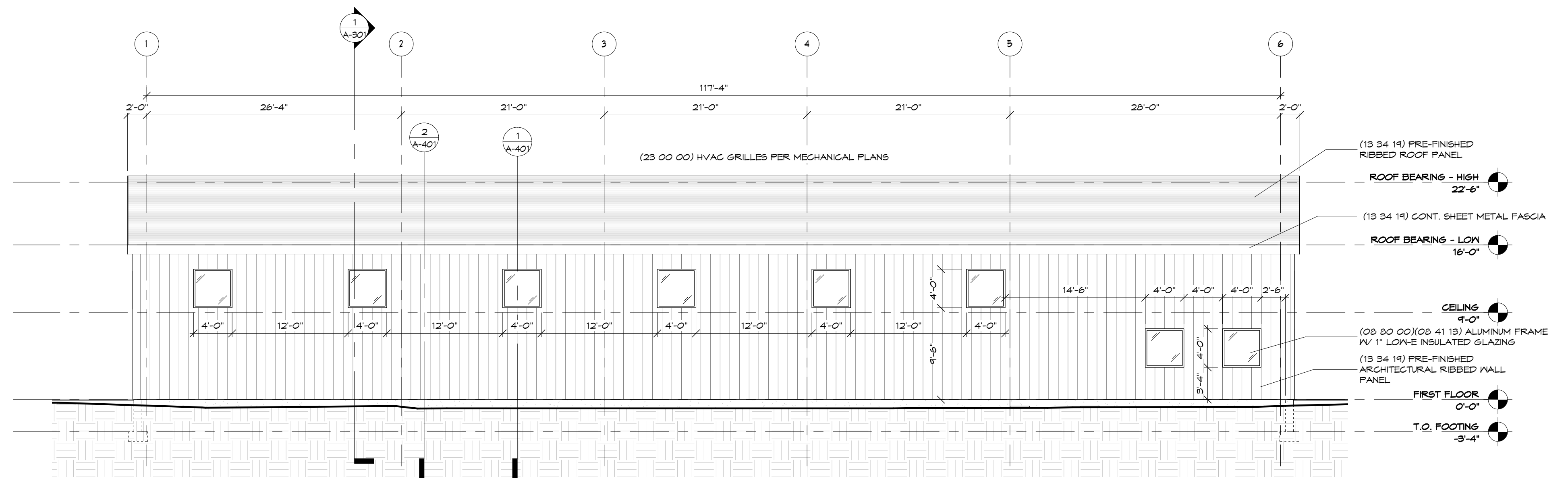
1 North Elevation 1/8" = 1'-0"
