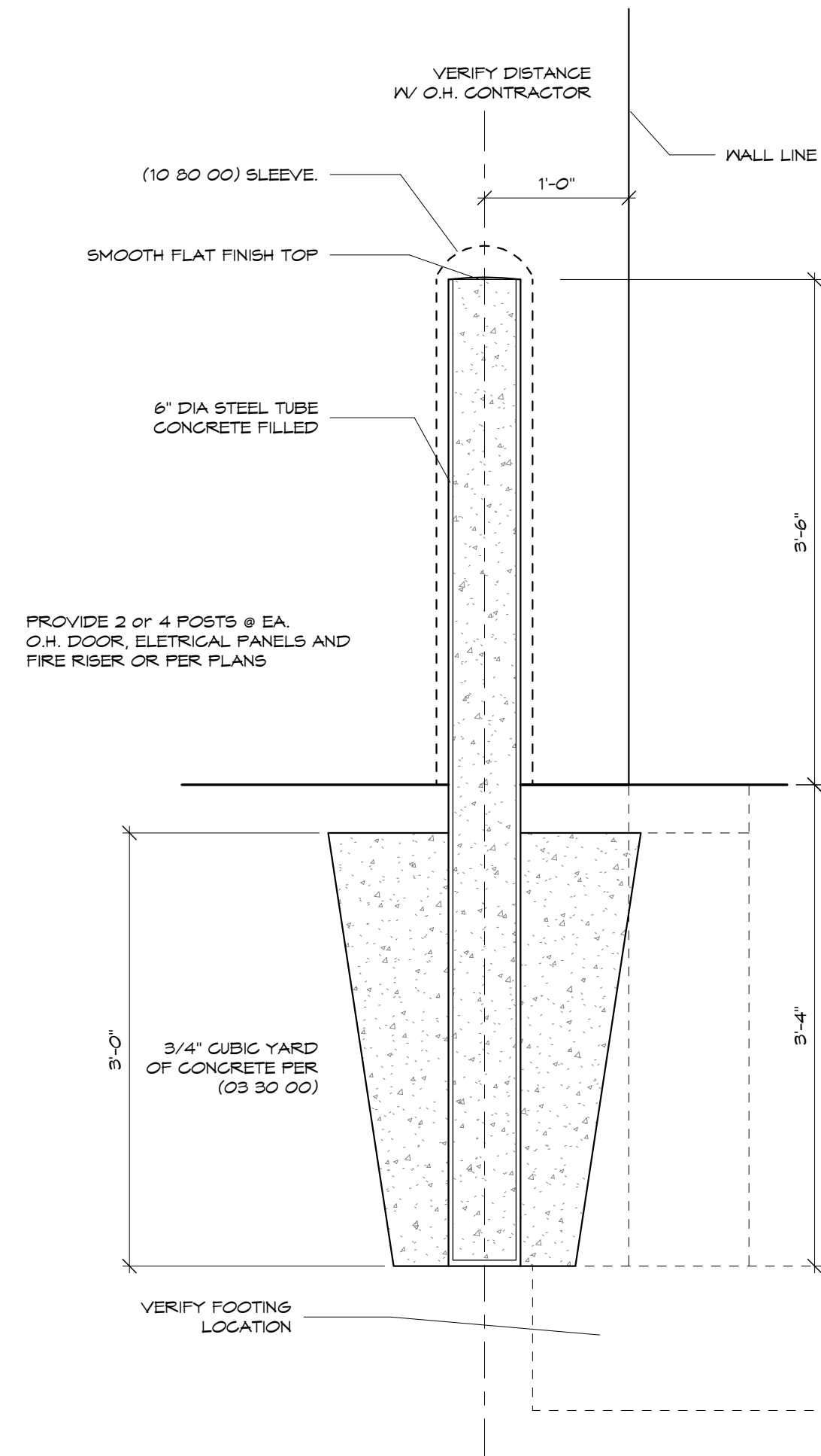
7 Concrete Bollard 1" = 1'-0"
