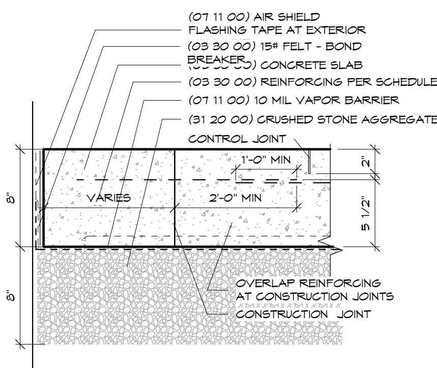
3 Concrete Slab - Type C 1 1/2" = 1'-0"
