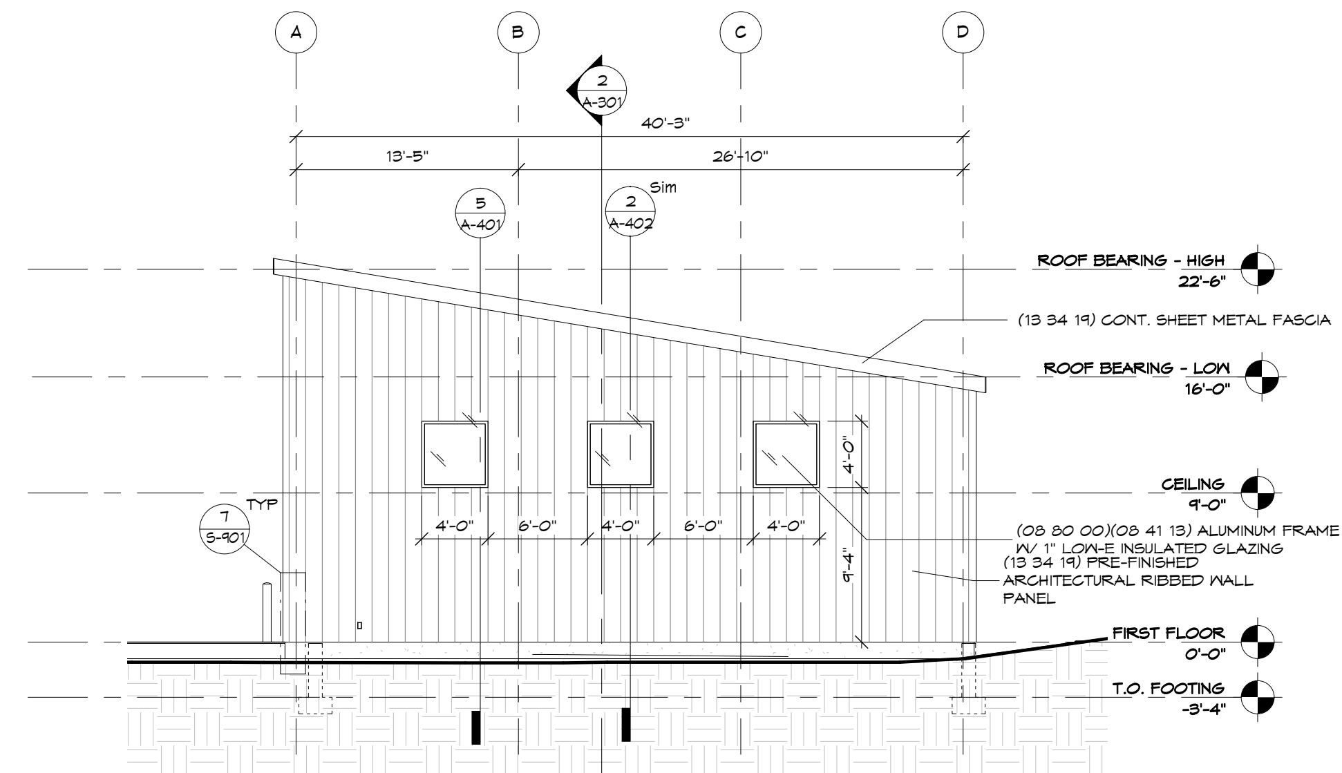
2 East Elevation 1/8" = 1'-0"
