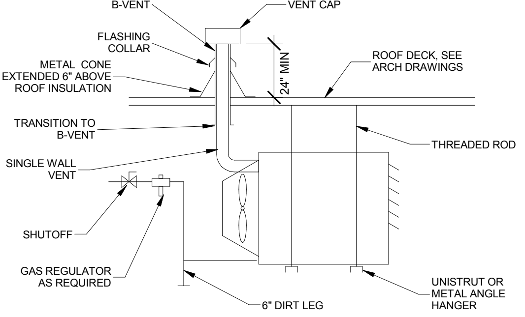
3 UNIT HEATER DETAIL SCALE: NO SCALE
