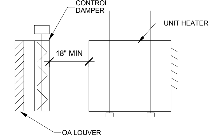
4 MAKE UP AIR LOUVER W/ UNIT HEATER DETAIL SCALE: NO SCALE
