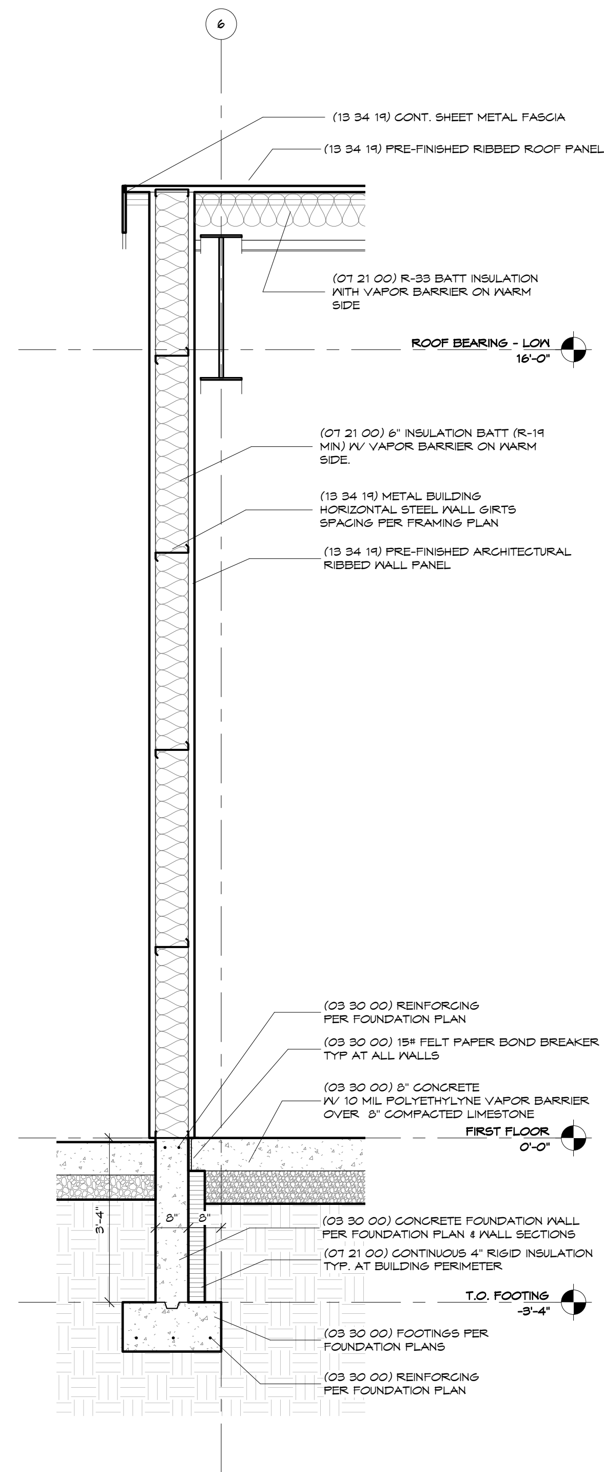
1 Wall Section 1/2" = 1'-0"
