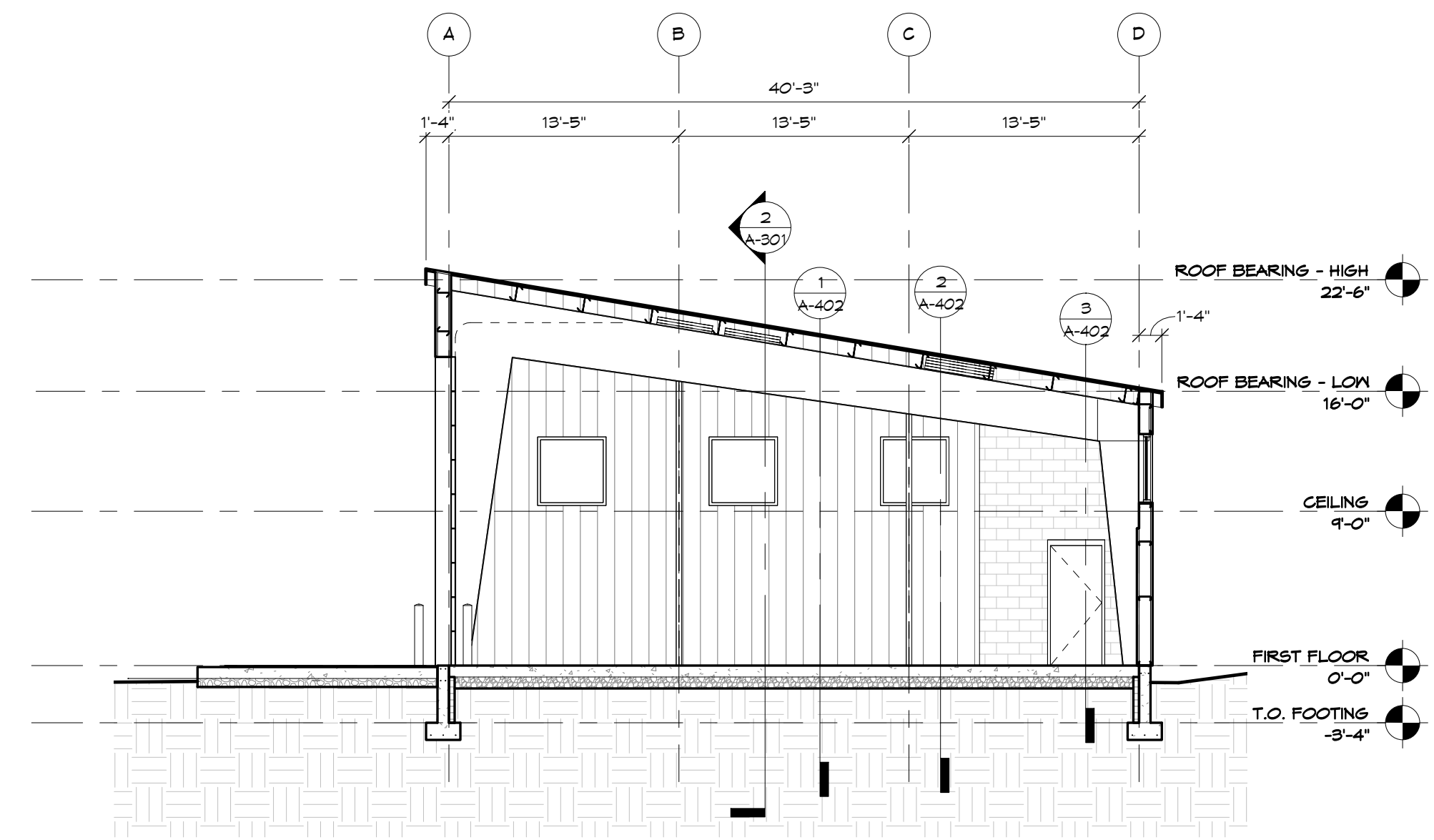
1 North-South Building Section 1/8" = 1'-0"
