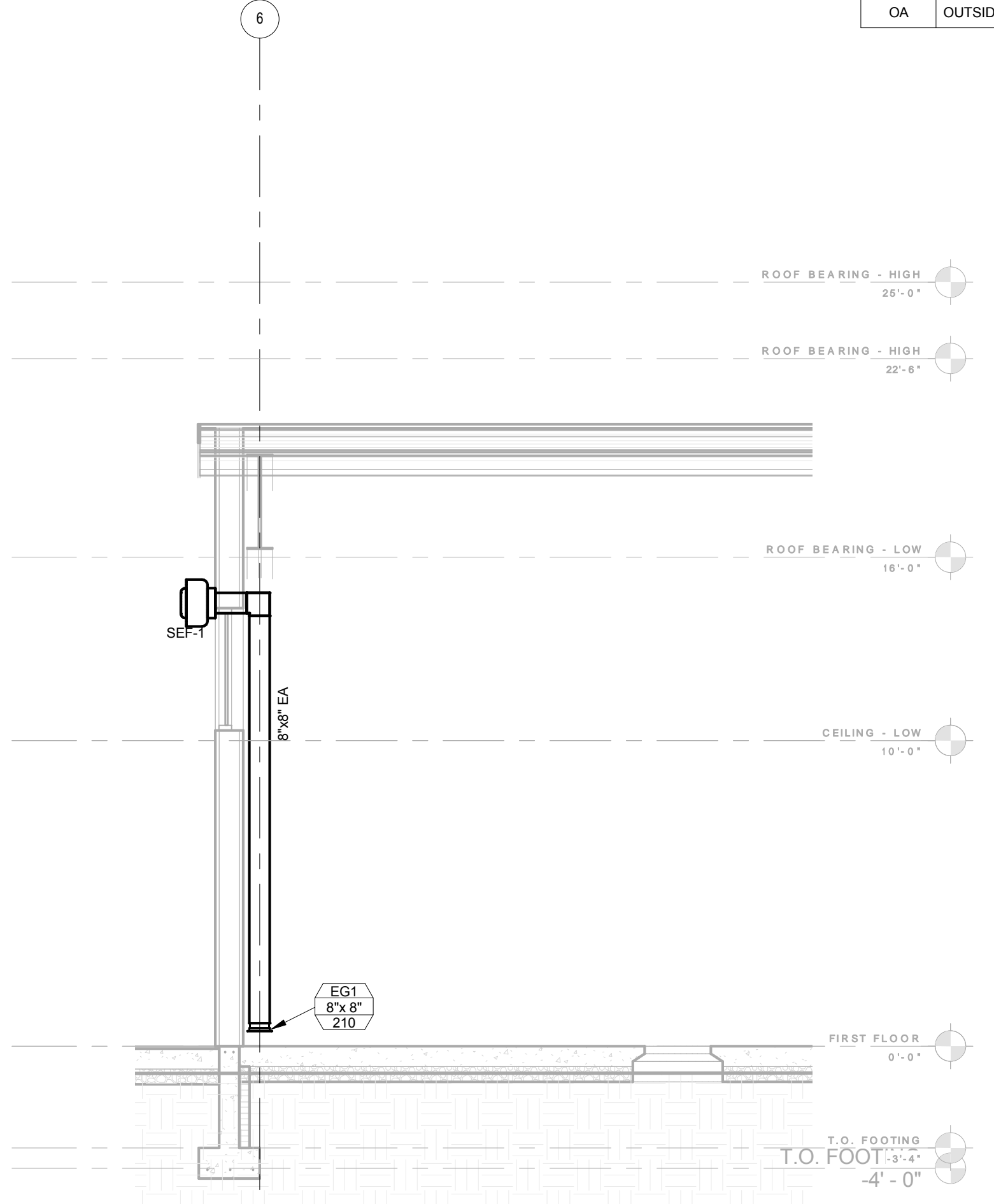
2 EXHAUST FAN SECTION SCALE: 1/4" = 1'-0"
