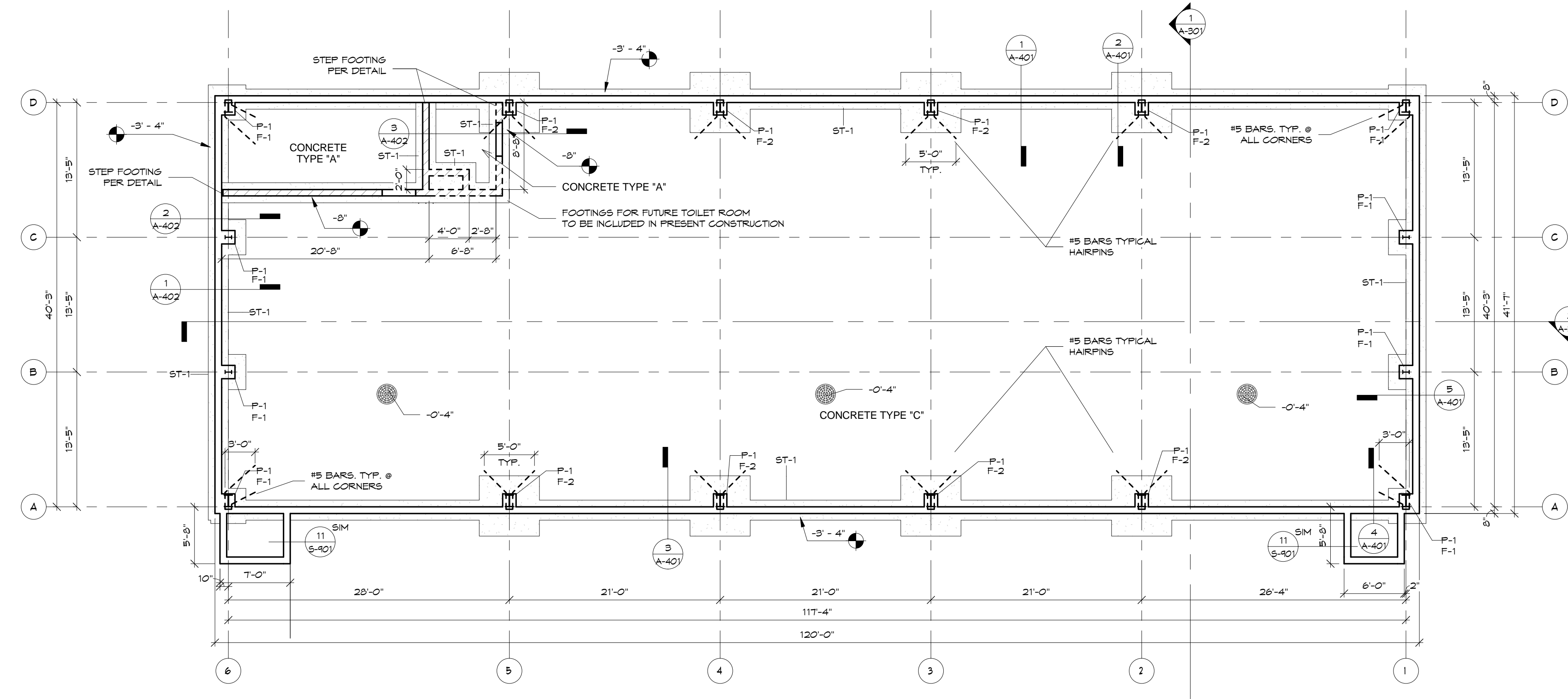
1 Foundation Plan 1/8" = 1'-0"
