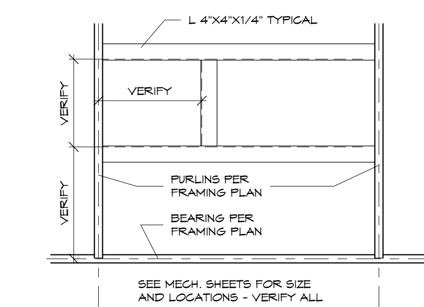
2 Framing at Roof Openings 1/2" = 1'-0"
