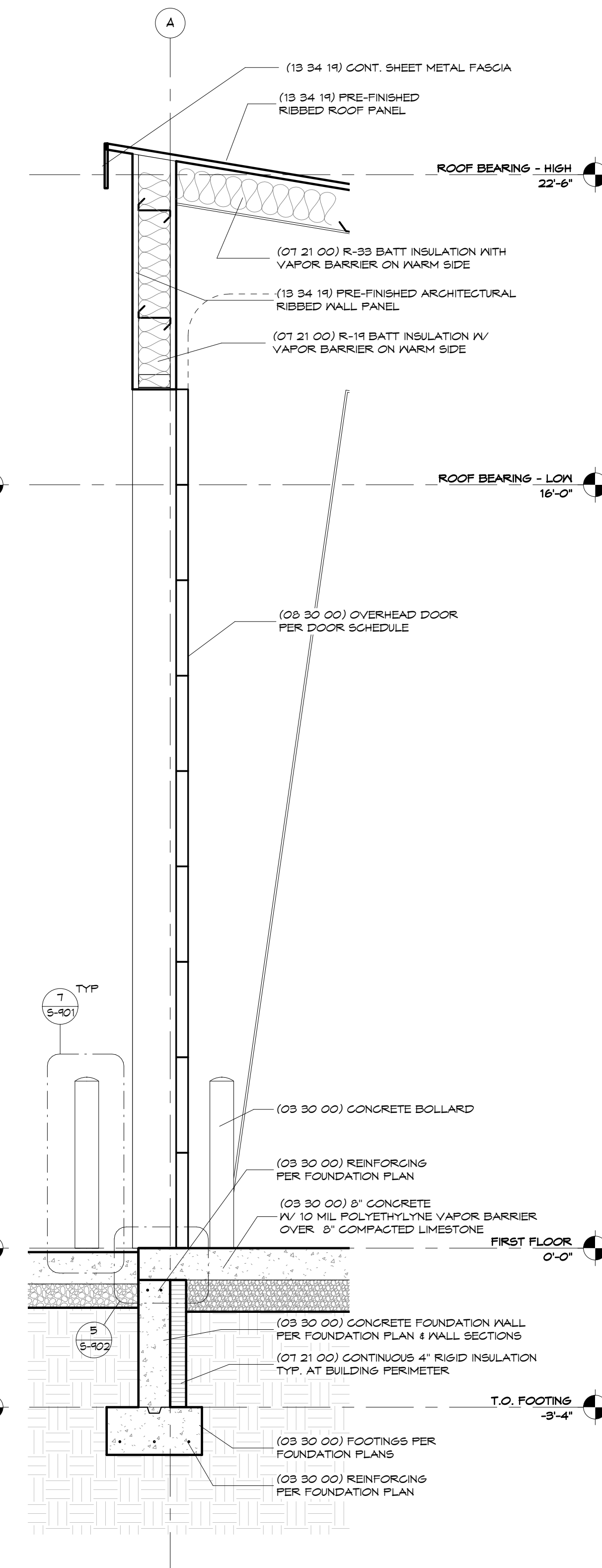
3 Wall Section 1/2" = 1'-0"
