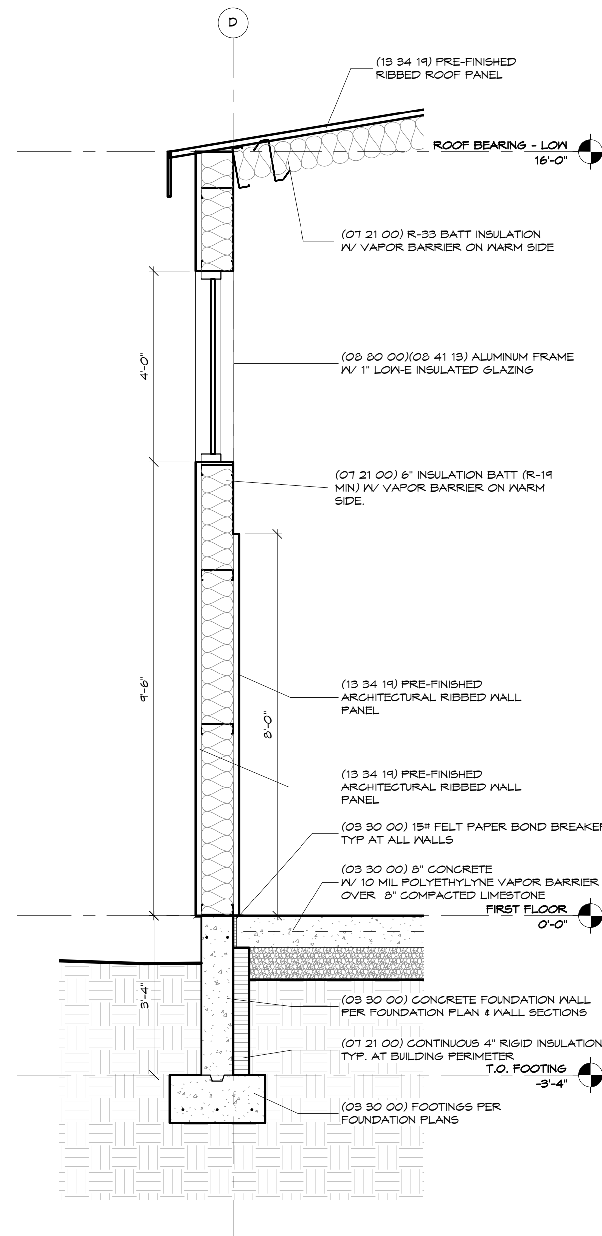
1 Wall Section 1/2" = 1'-0"
