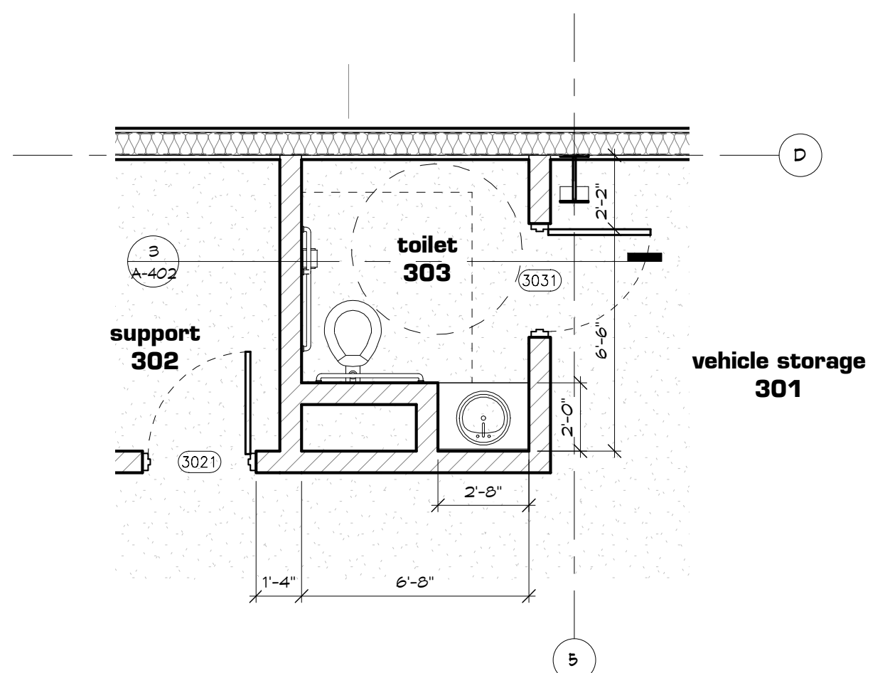
3 Future Enlarged Toilet Rooms 1/4" = 1'-0"
