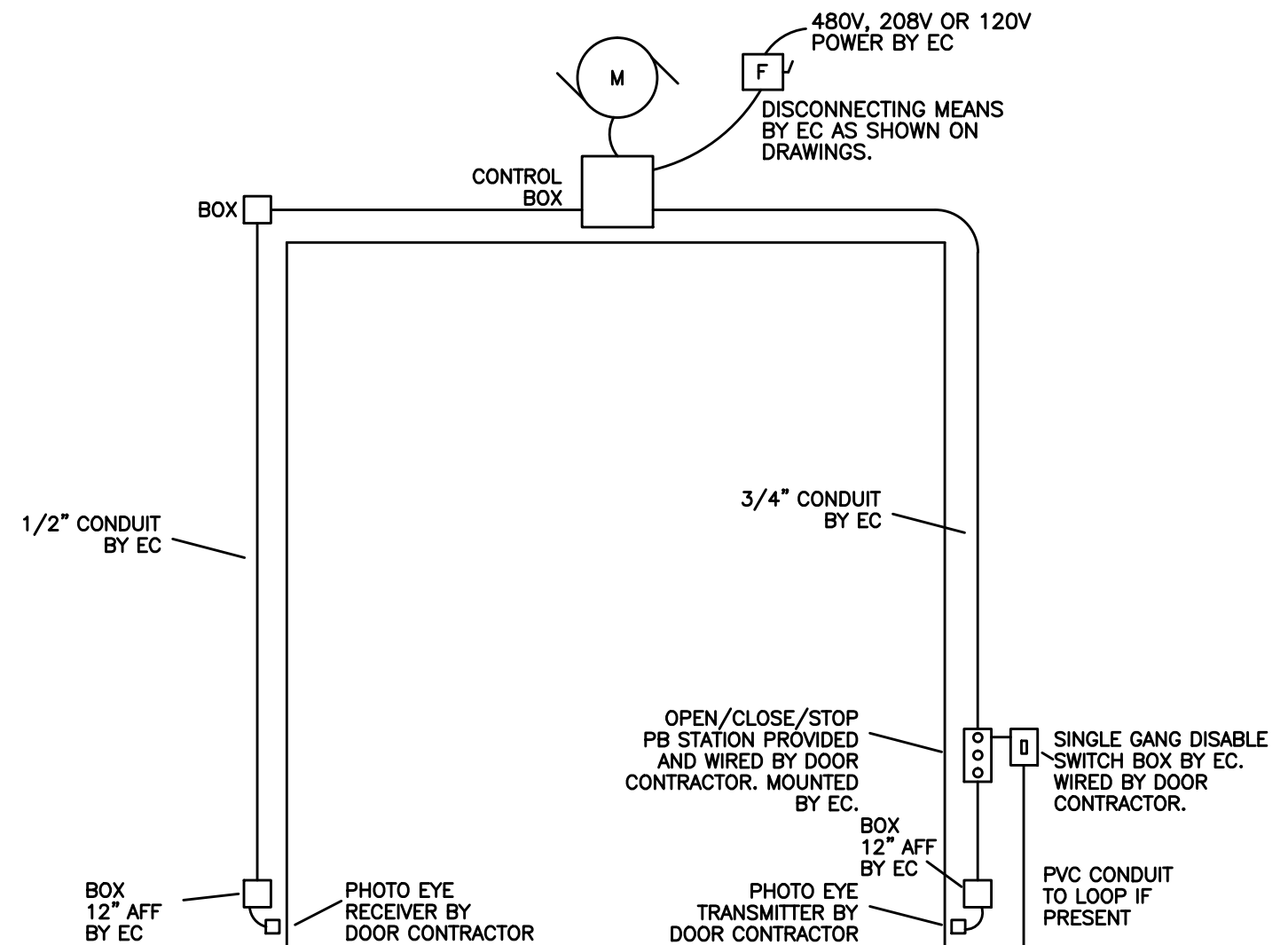
1 TYPICAL: OVERHEAD DOOR
