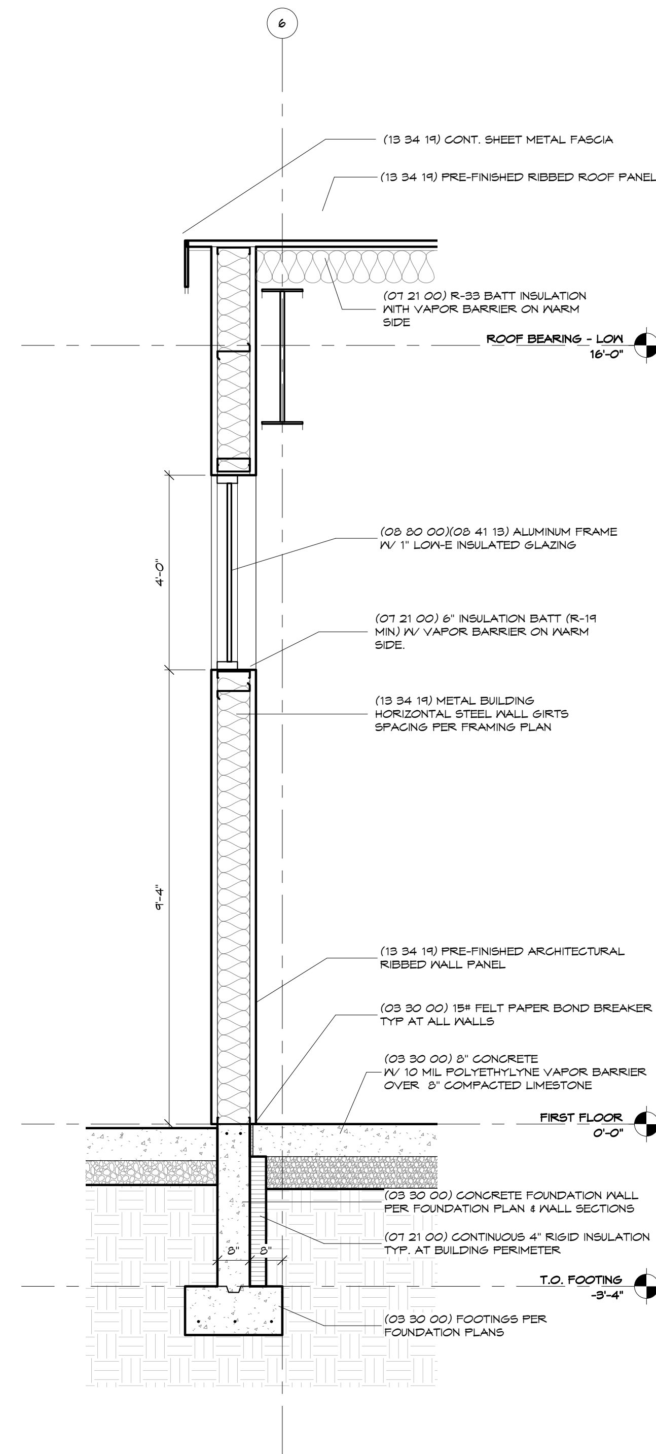
2 Wall Section 1/2" = 1'-0"
