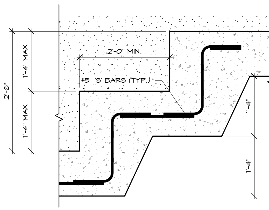
5 Footing Step - Typ. 3/4" = 1'-0"
