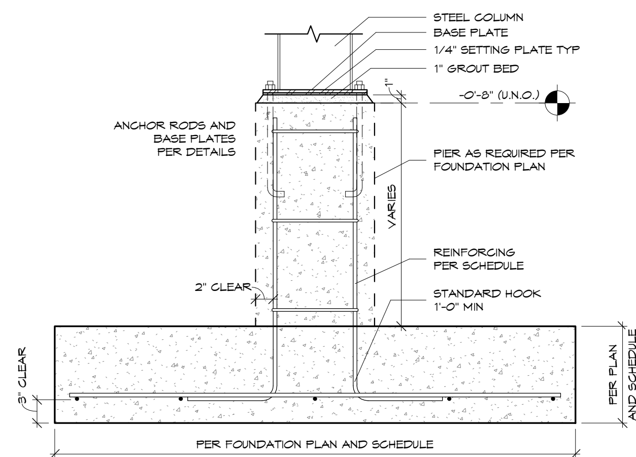
9 Pad Footing - Typ 1" = 1'-0"
