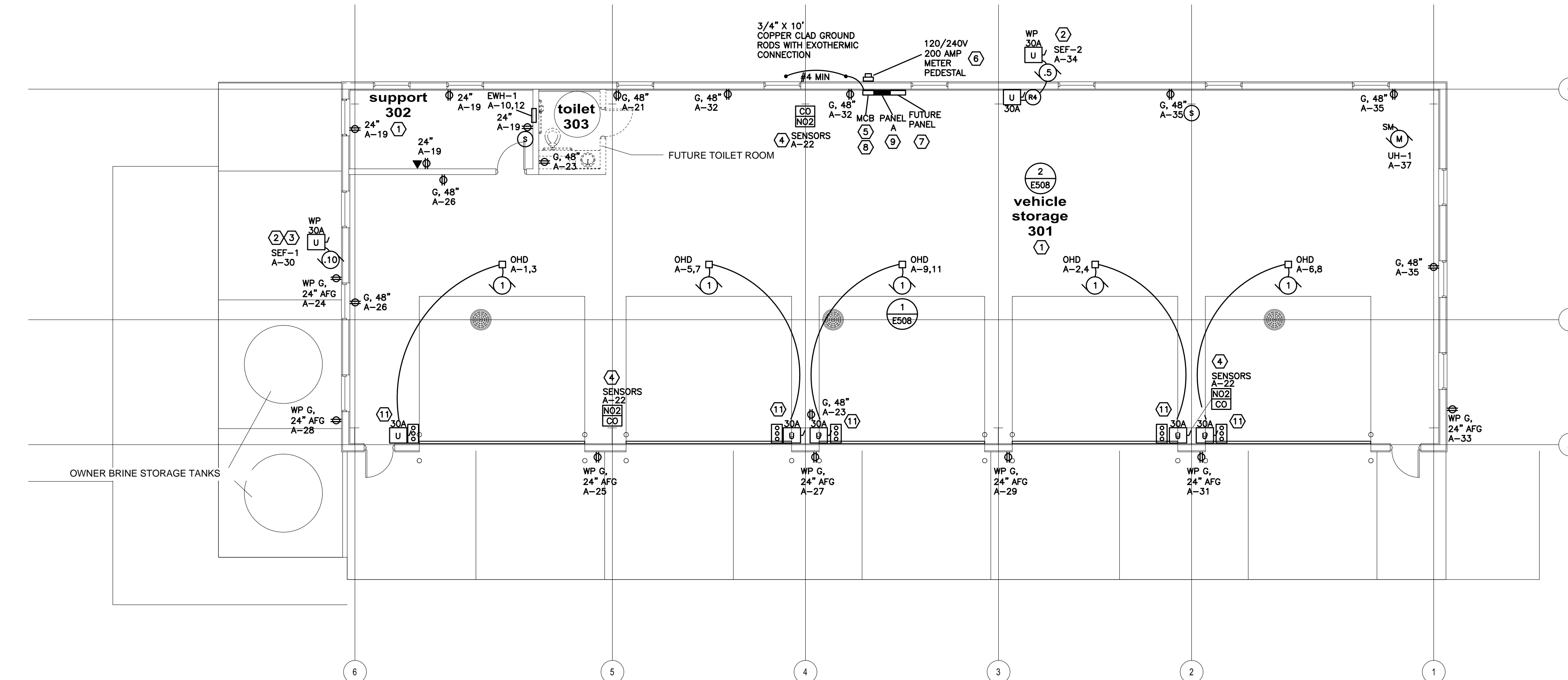
2 Satellite Building Power and Systems Plan 1/8" = 1'-0"
