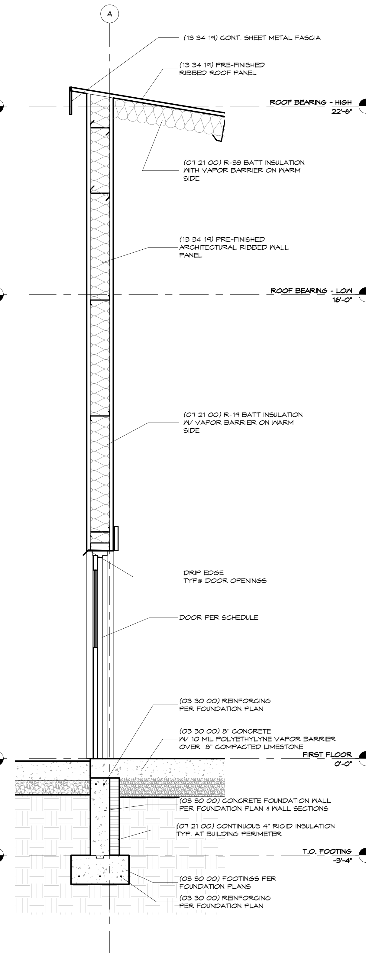
4 Wall Section 1/2" = 1'-0"
