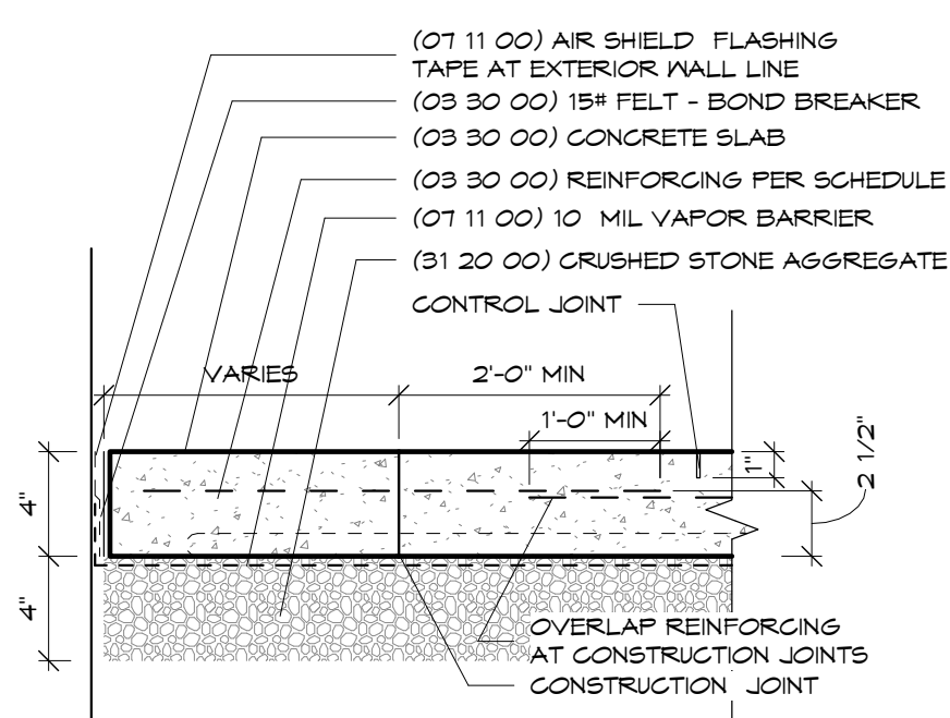
2 Concrete Slab - Type A 1 1/2" = 1'-0"
