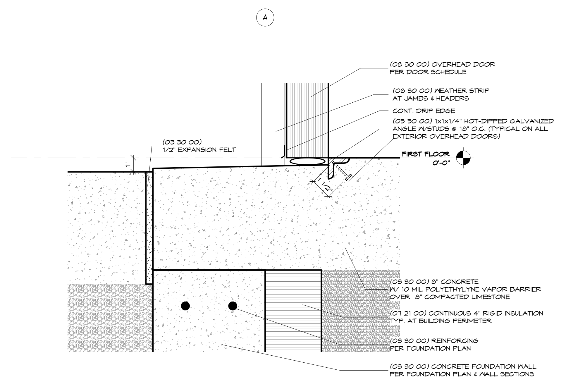
5 OH Door Threshold 3" = 1'-0"
