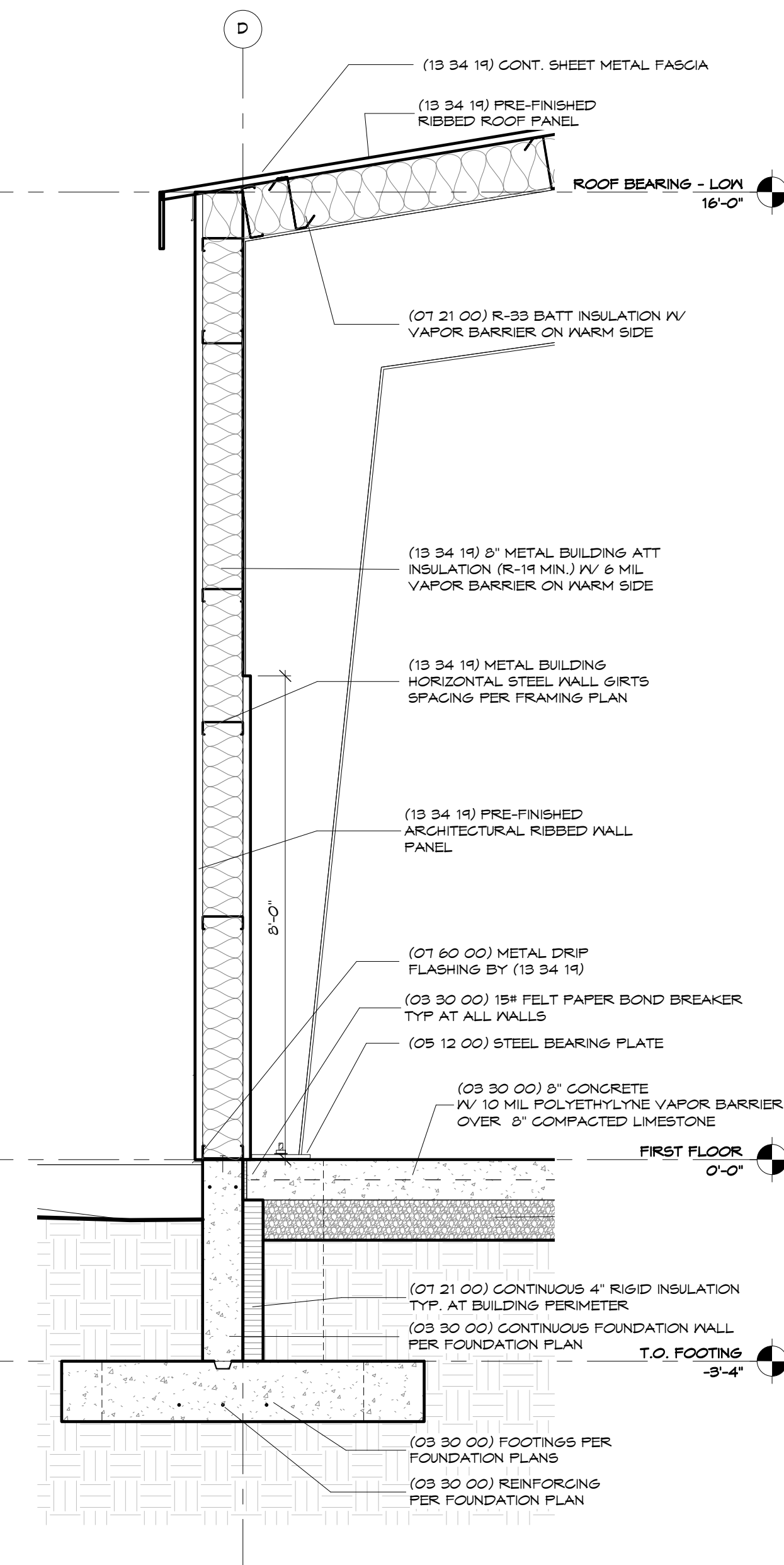
2 Wall Section 1/2" = 1'-0"
