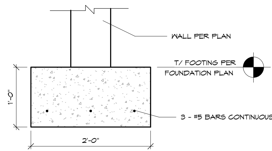
4 Strip Footing - Typ 1" = 1'-0"
