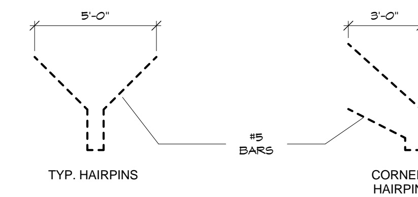
6 Typ. Hairpins 1/4" = 1'-0"
