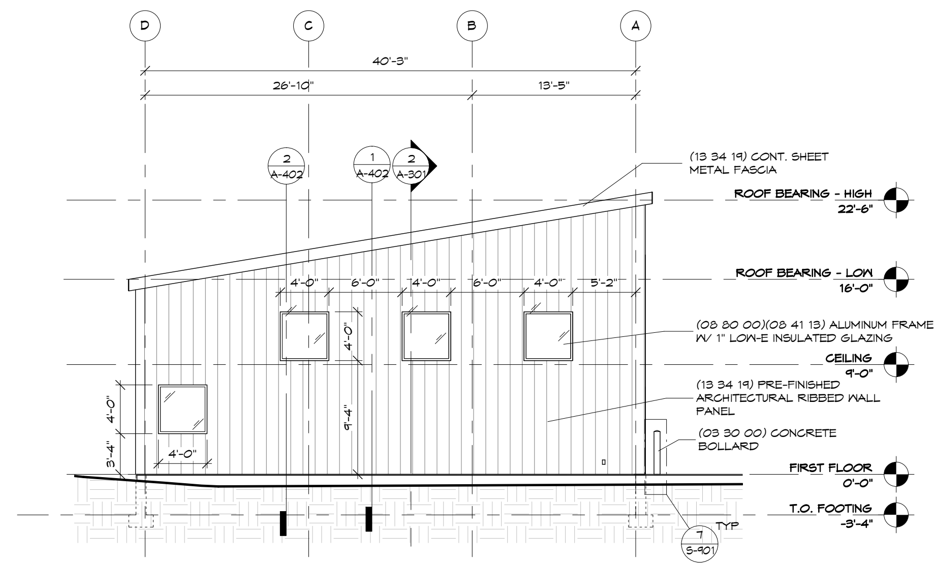
4 West Elevation 1/8" = 1'-0"
