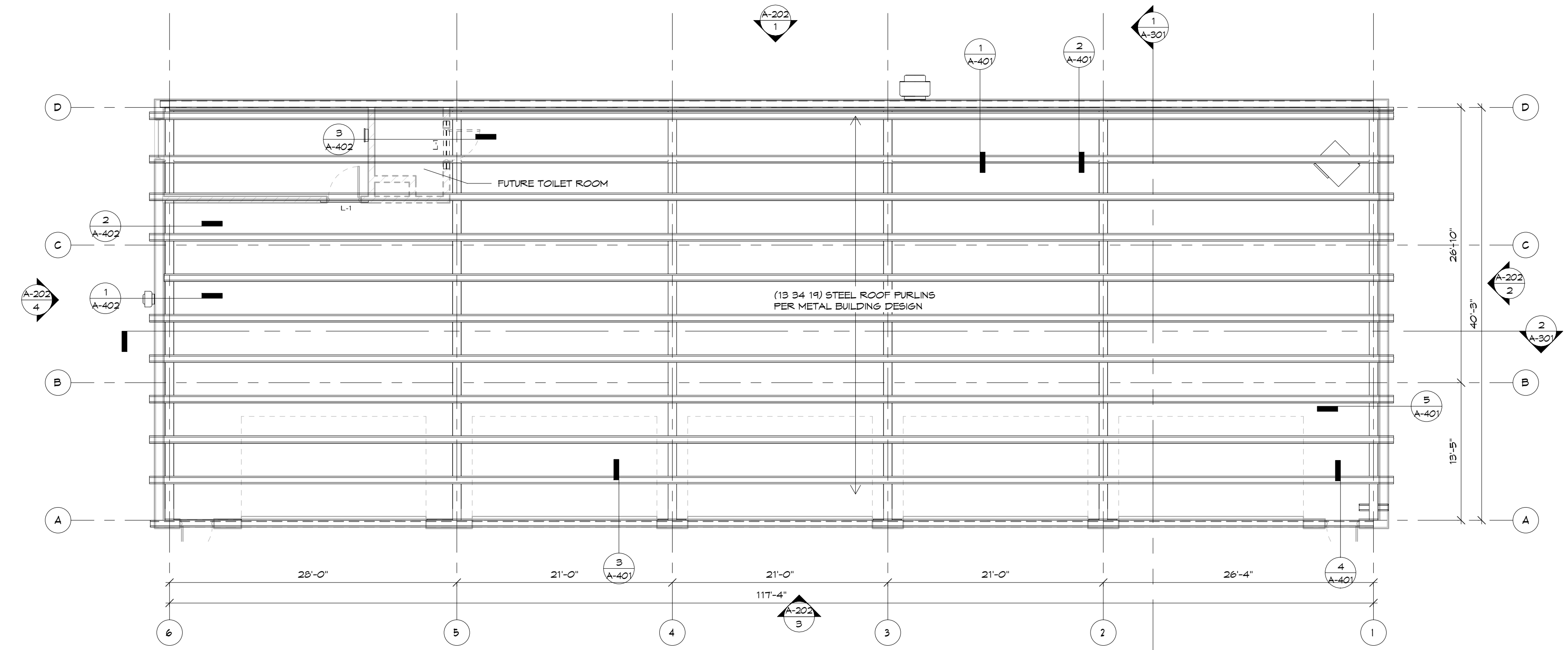
1 Roof Framing Plan 1/8" = 1'-0"
