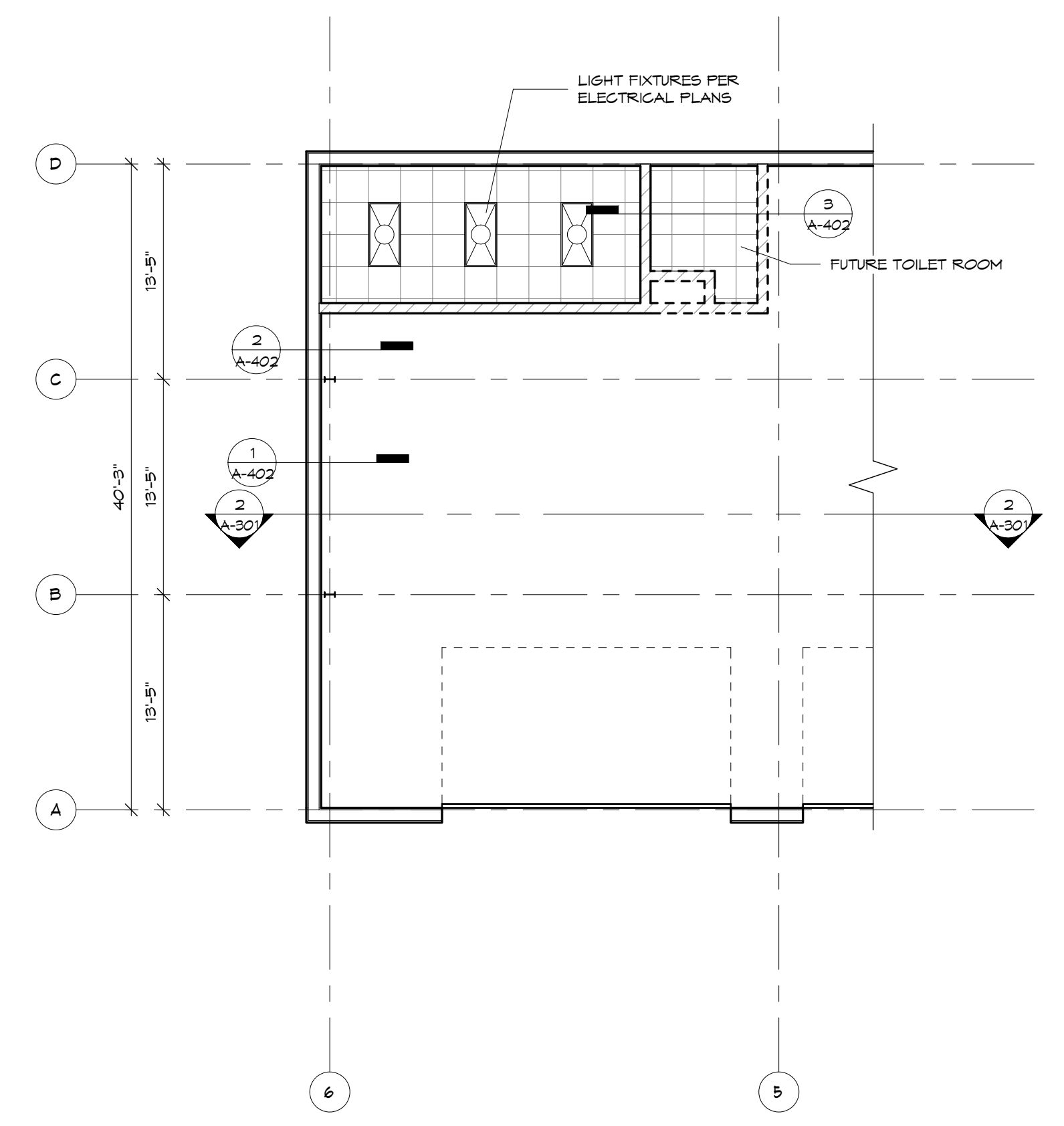
4 Reflected Ceiling Plan 1/8" = 1'-0"
