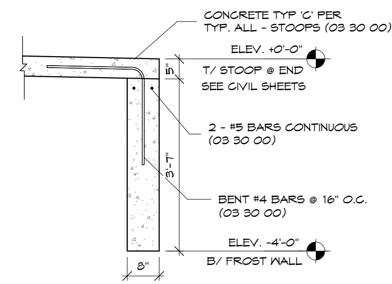
11 Stoop Frost Wall 1/2" = 1'-0"
