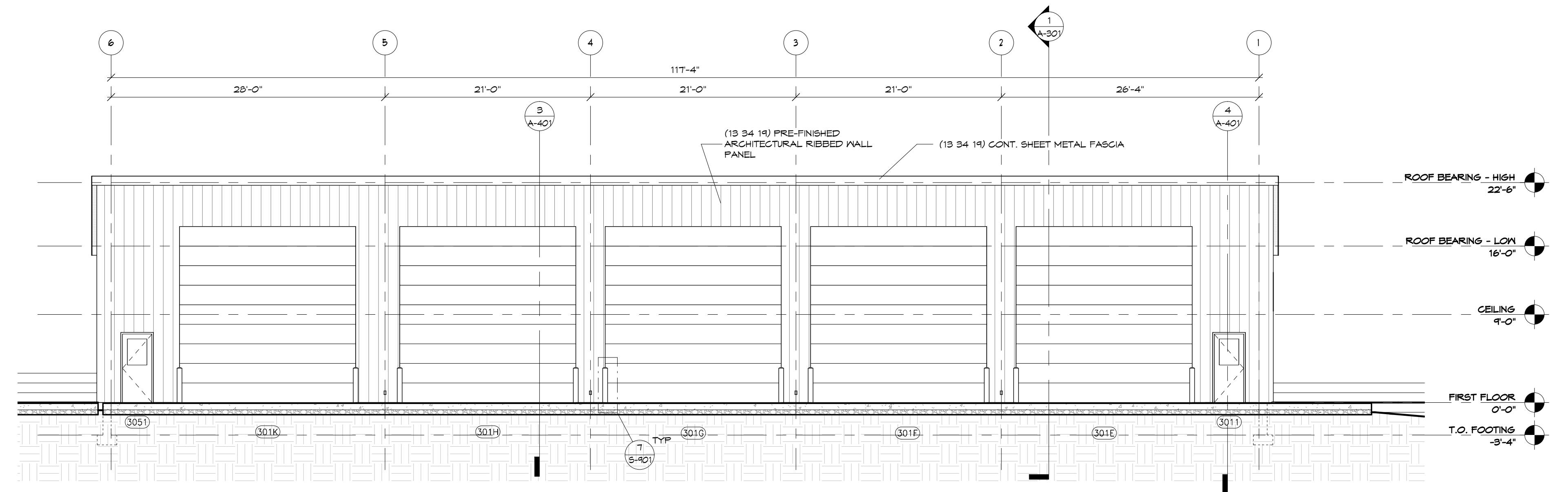
3 South Elevation 1/8" = 1'-0"
