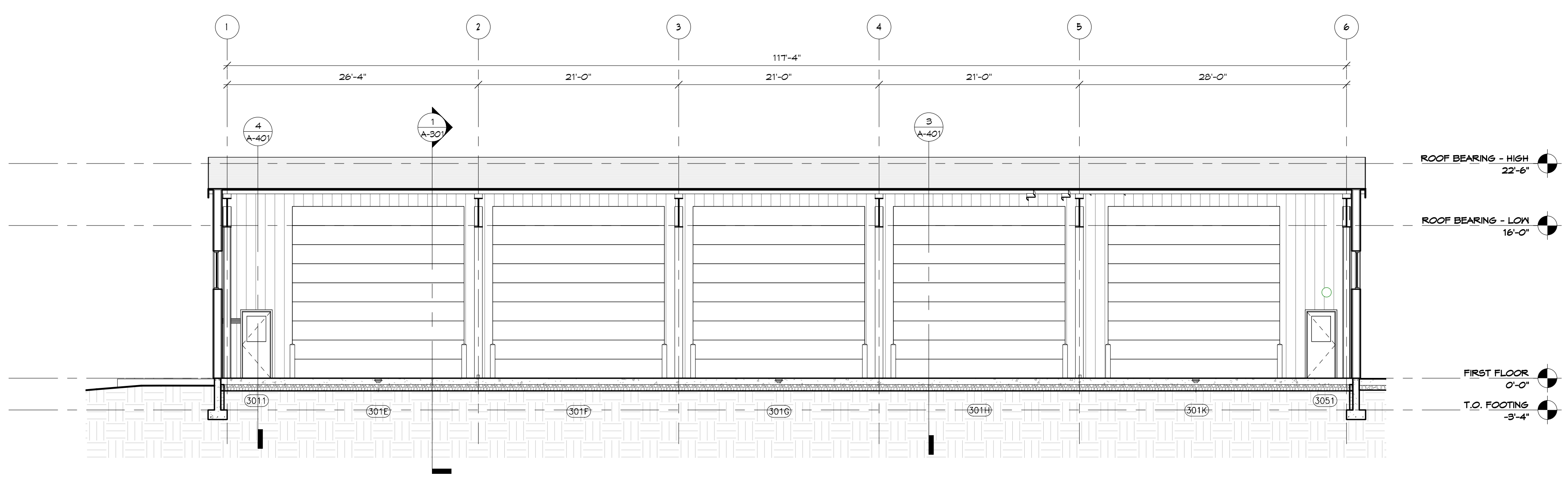
2 East-West Building Section 1/8" = 1'-0"
