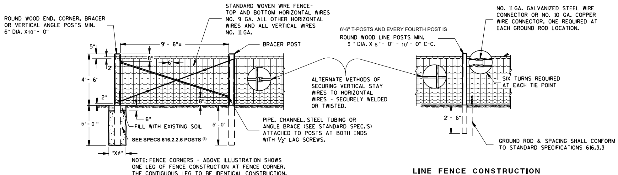
LINE FENCE CONSTRUCTION
