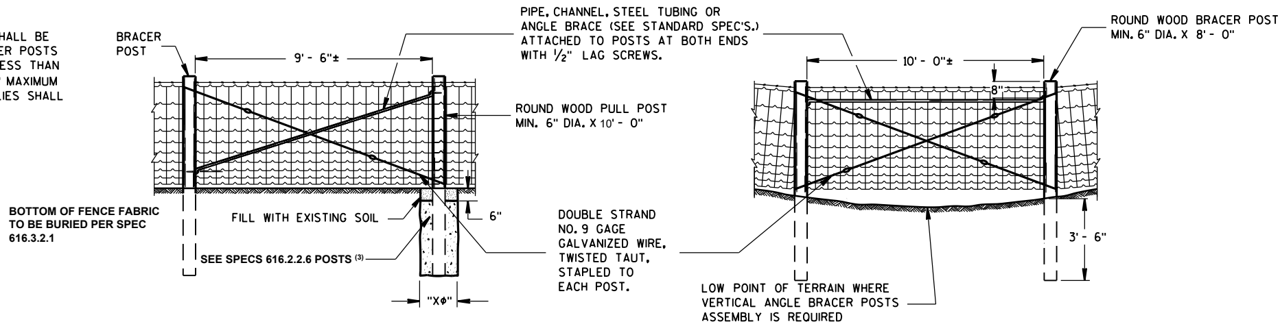
PULL OR STRETCHER POSTS ASSEMBLY
