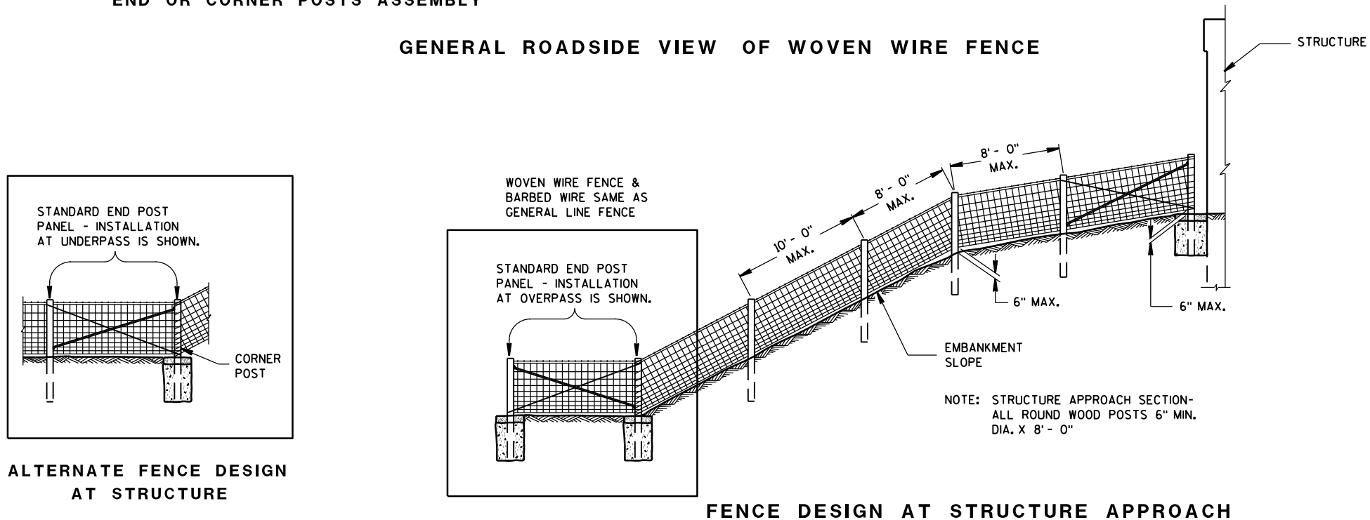
FENCE DESIGN AT STRUCTURE APPROACH
