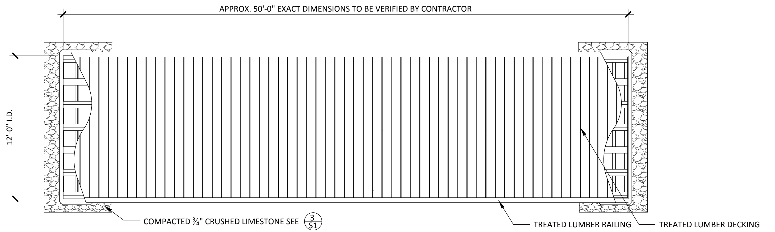
1 S1 BRIDGE PLAN NTS
