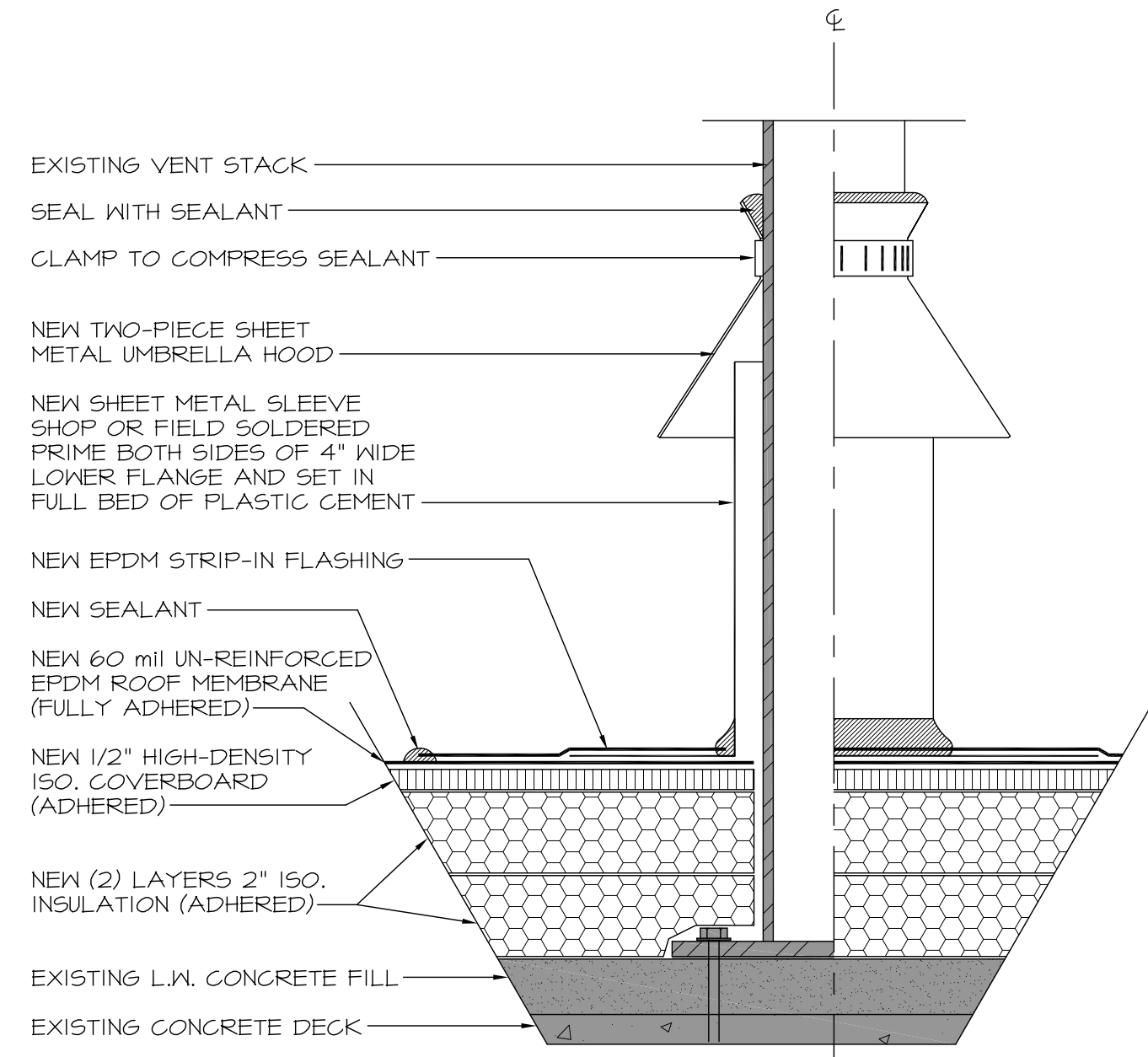
12 PIPE PENETRATION DETAIL 3 SCALE: 3/8"=1'-0"
