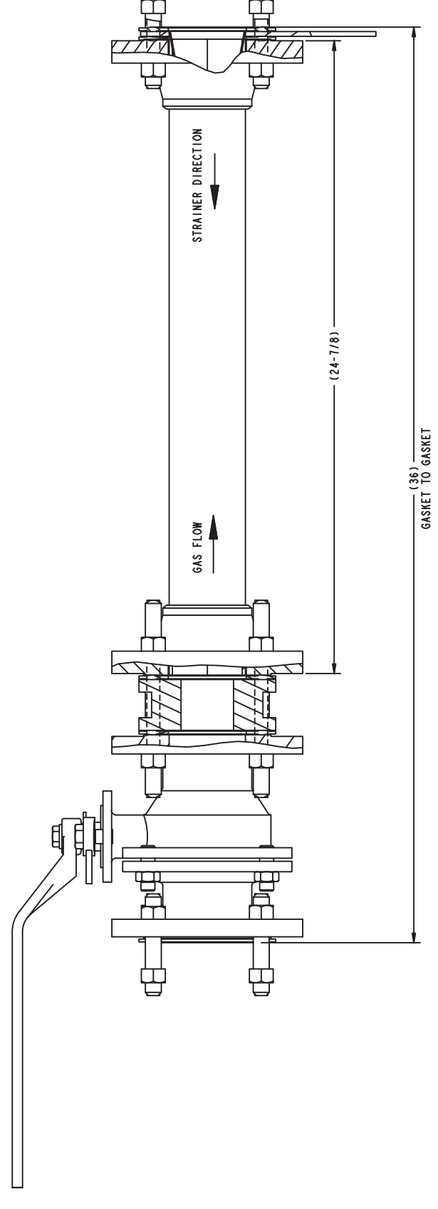
HOSE FLEX PIECE
