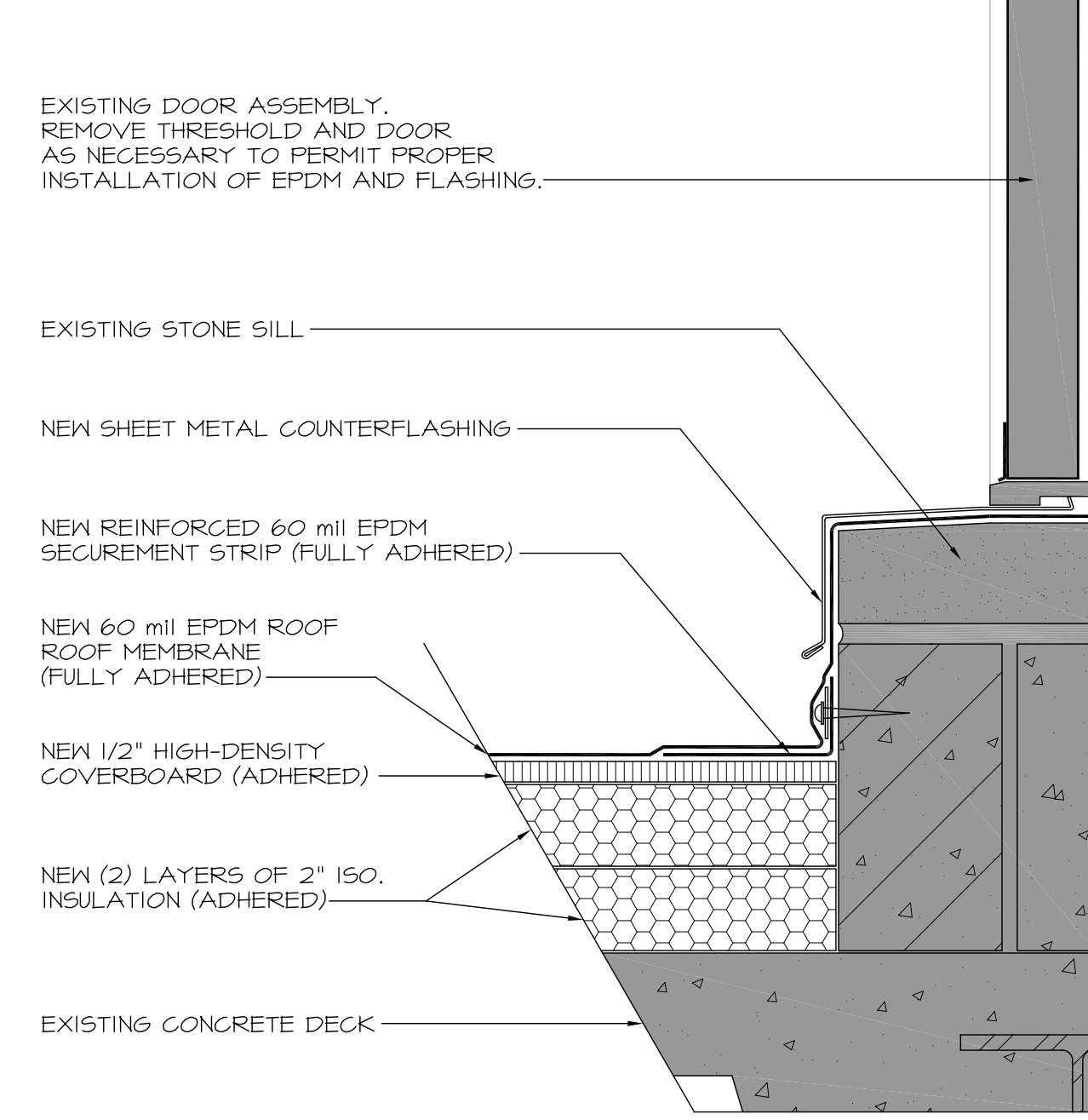
4 DOOR THRESHOLD DETAIL 2 SCALE: 3"=1'-0"
