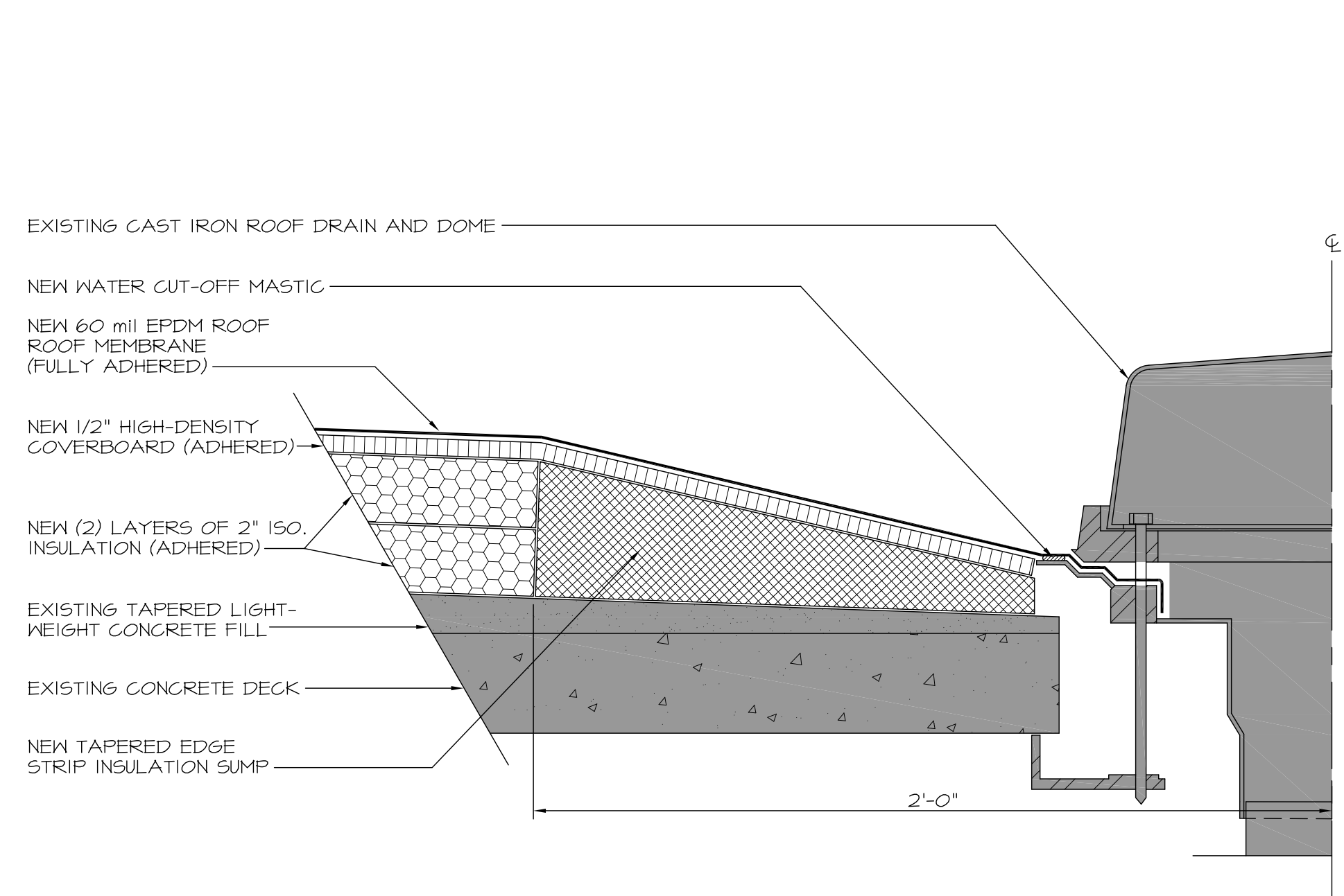
8 ROOF DRAIN DETAIL 2 SCALE: 3"=1'-0"
