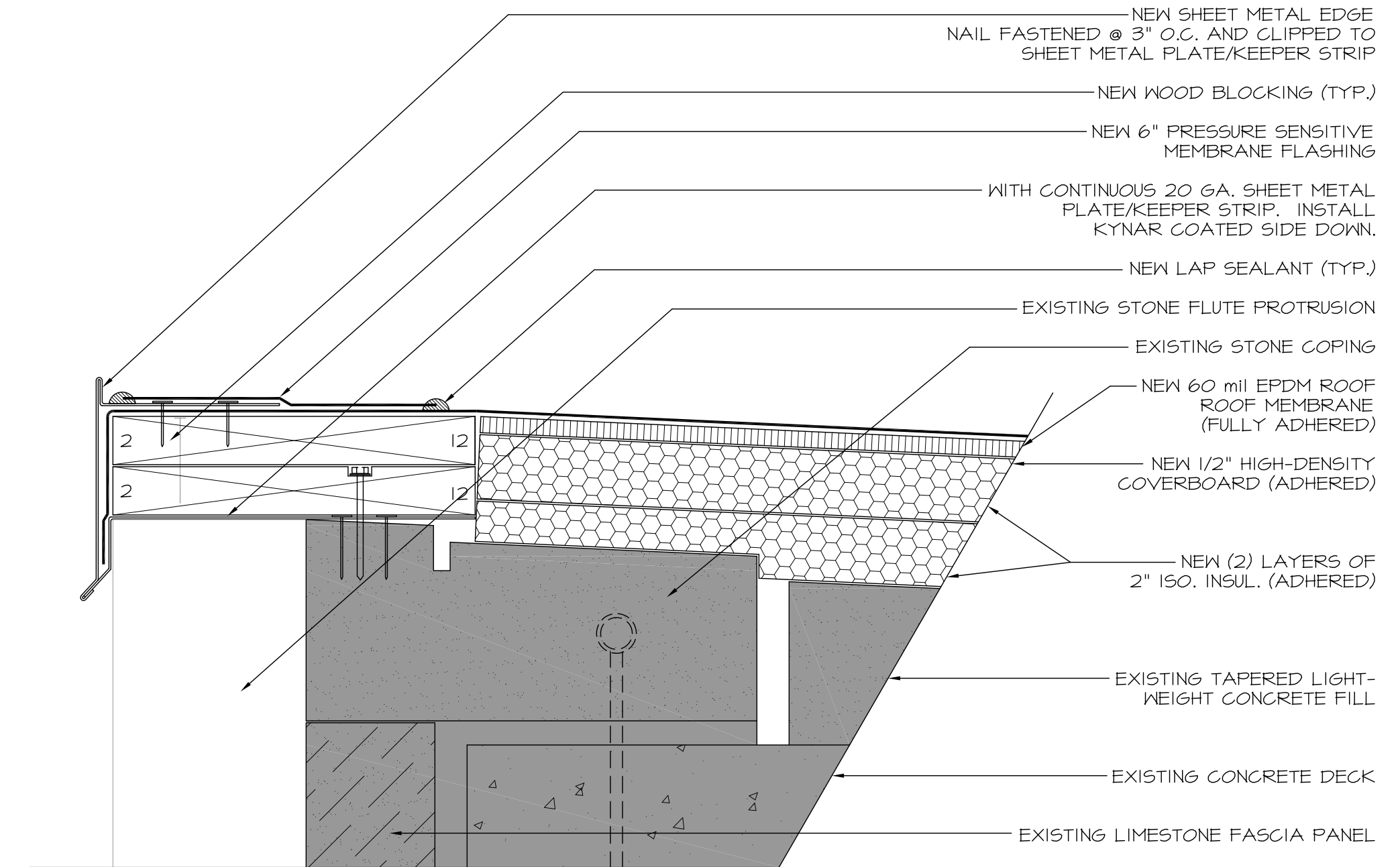
7 EDGE FLASHING AT FLUTE DETAIL 2 SCALE: 3"=1'-0"
