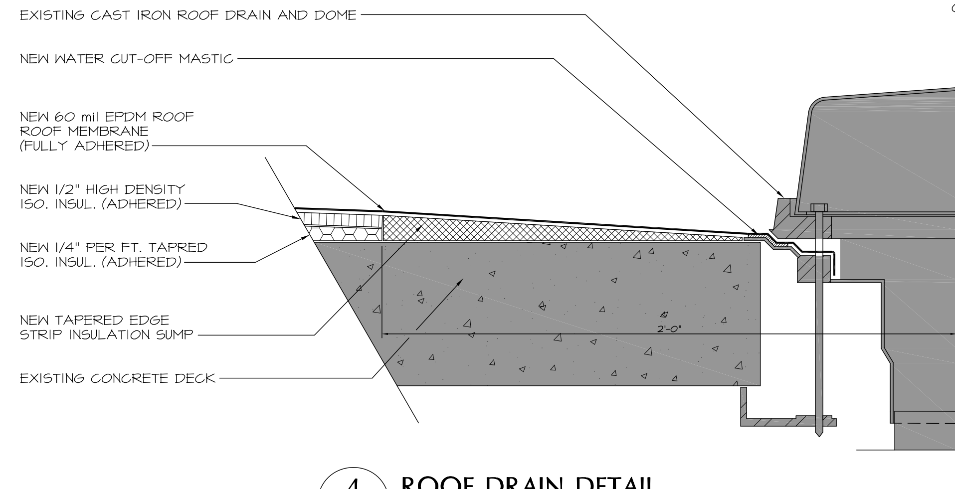
4 ROOF DRAIN DETAIL 2 SCALE: 3"=1'-0"
