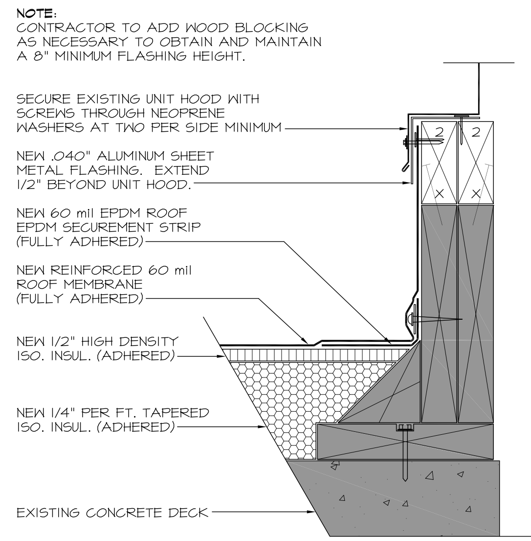
6 HVAC UNIT CURB DETAIL 2 SCALE: 3"=1'-0"
