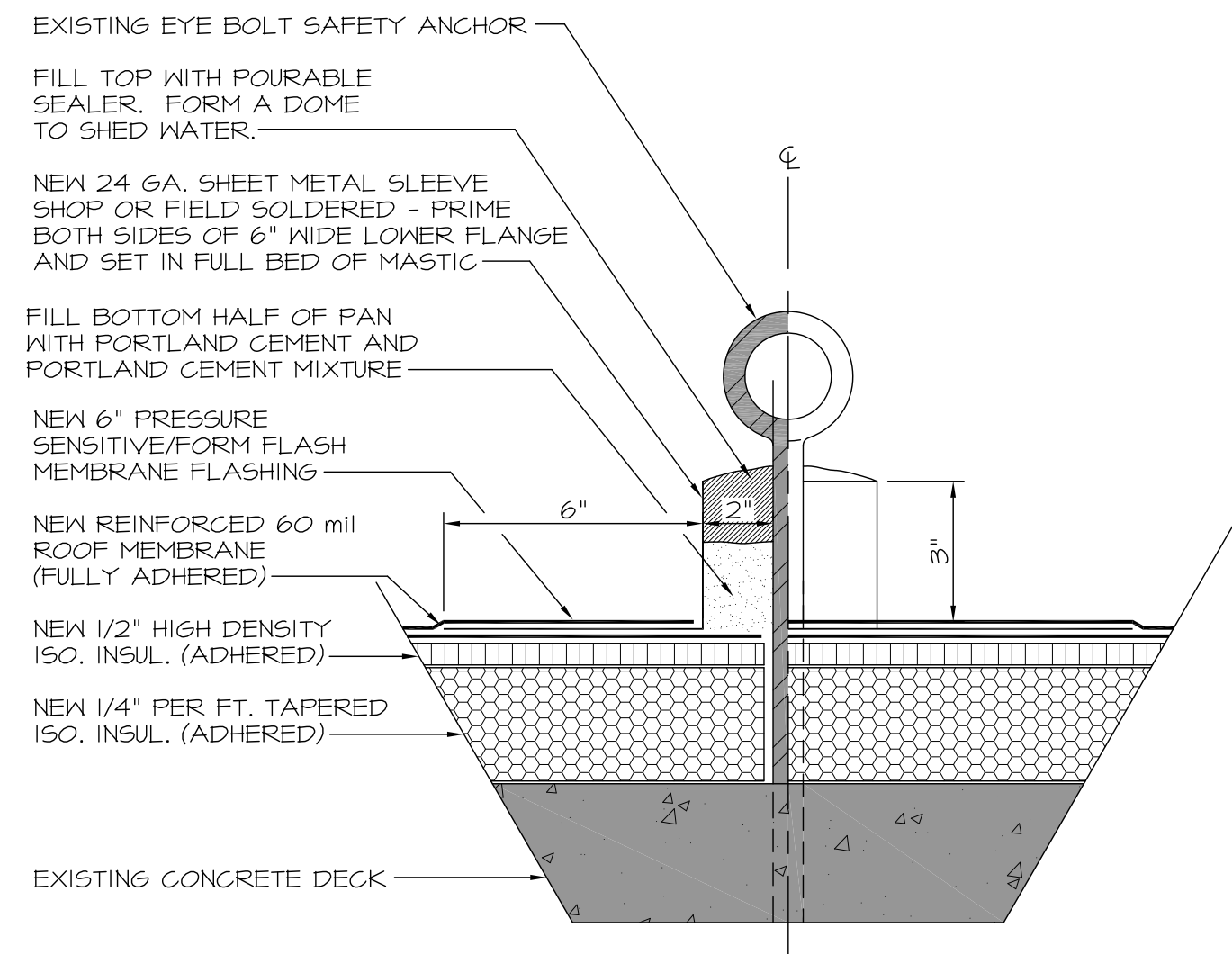
8 SAFETY ANCHOR FLASHING DETAIL 2 SCALE: 3"=1'-0"
