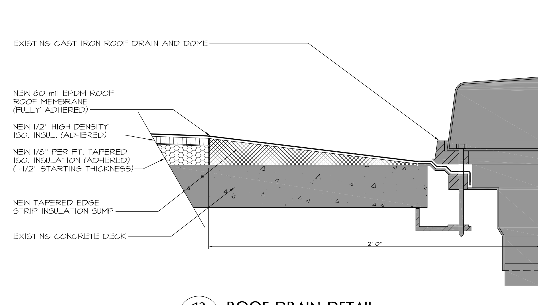
13 ROOF DRAIN DETAIL 3 SCALE: 3"=1'-0"
