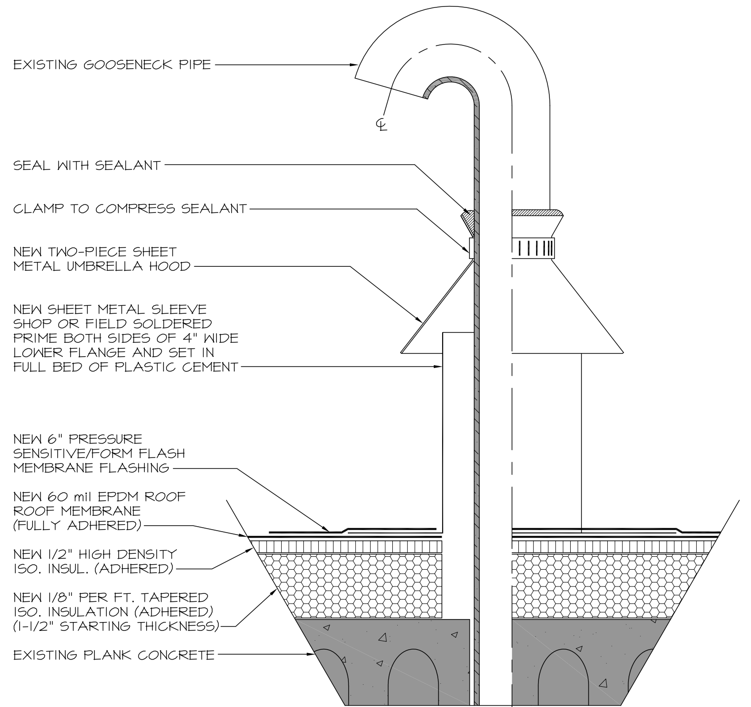
15 GOOSENECK VENT DETAIL 3 SCALE: 3"=1'-0"
