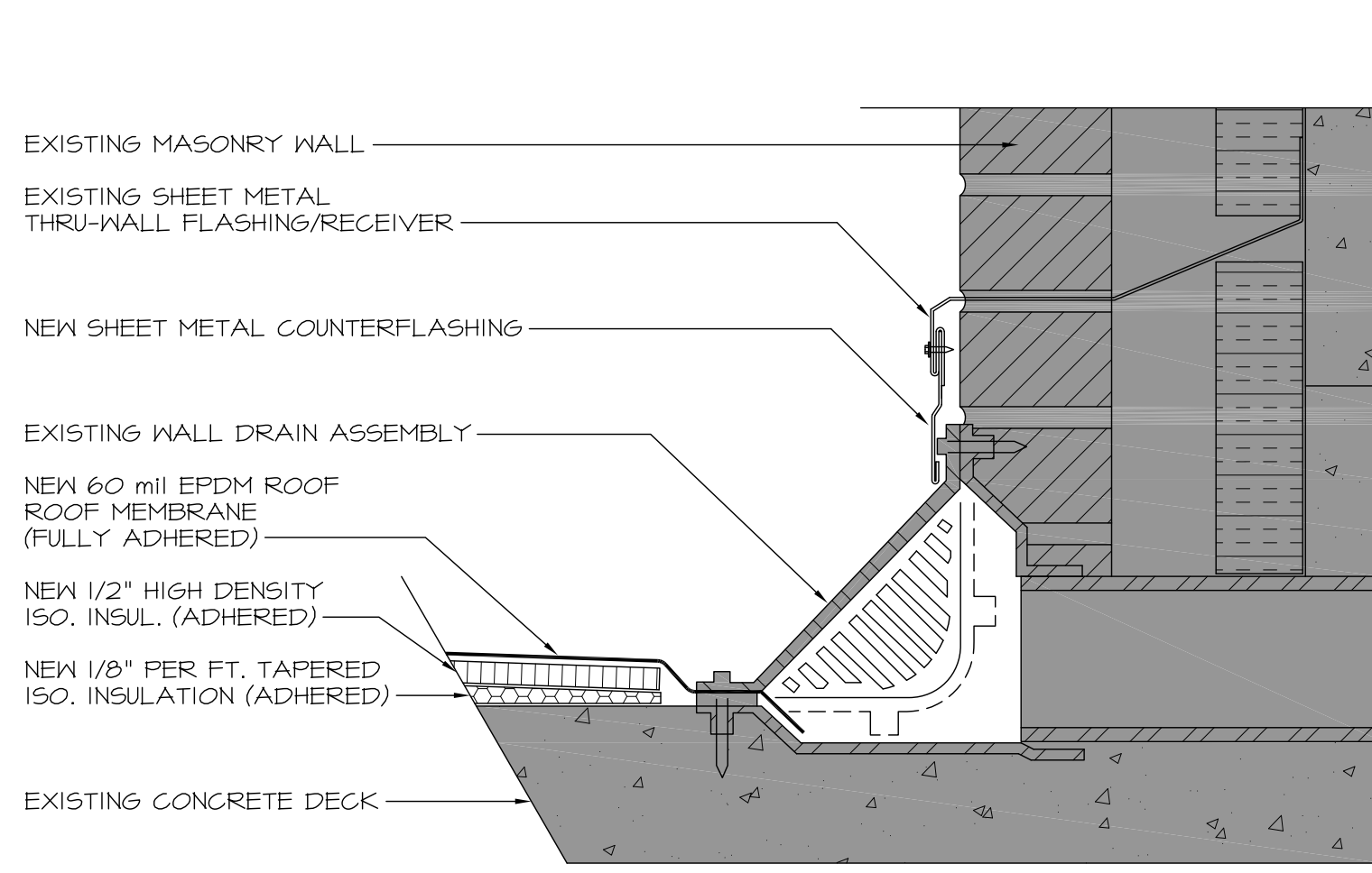
11 WALL DRAIN FLASHING DETAIL 3 SCALE: 3"=1'-0"
