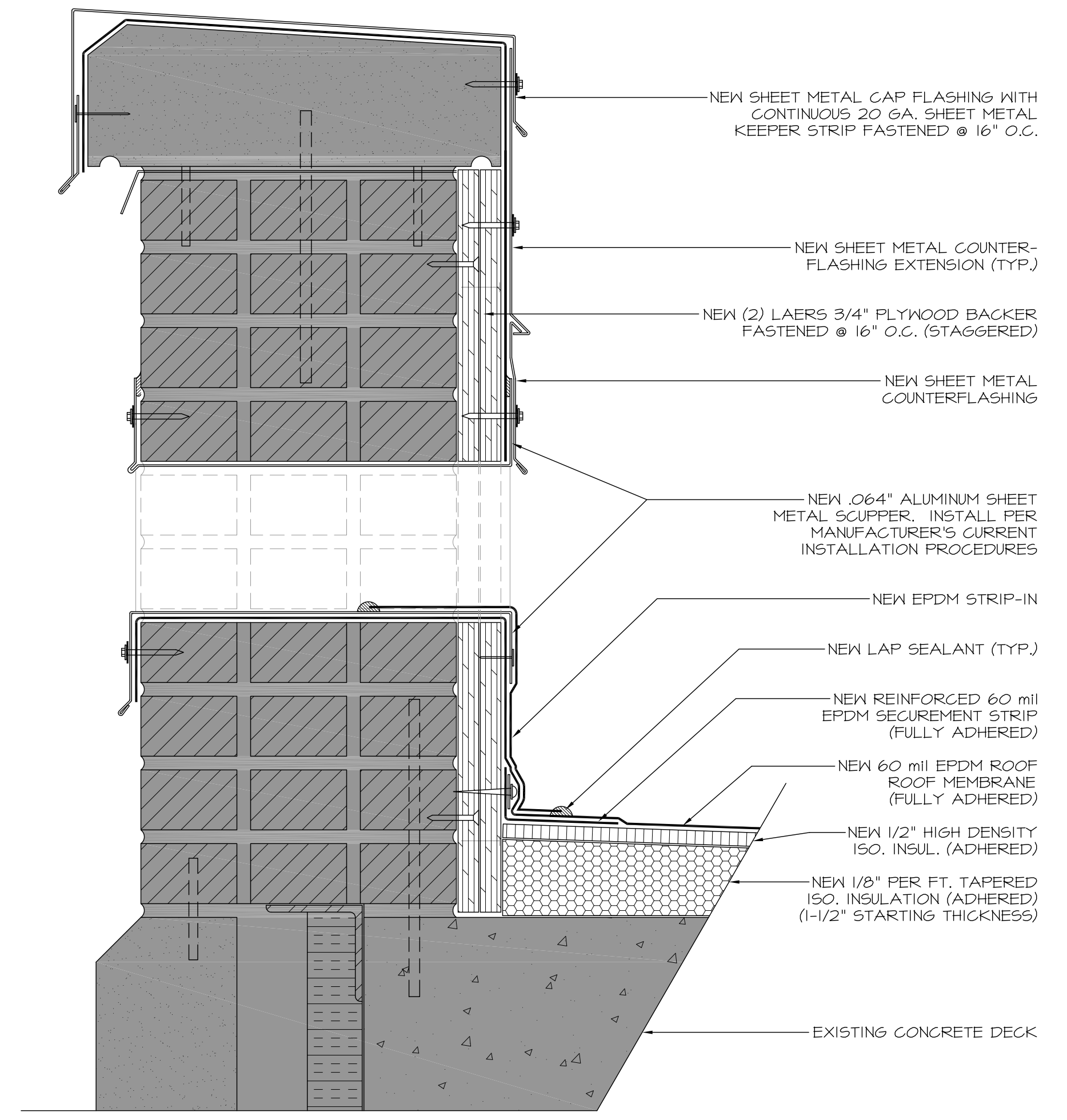
3 1 OVERFLOW SCUPPER DETAIL SCALE: 3"=1'-0"
