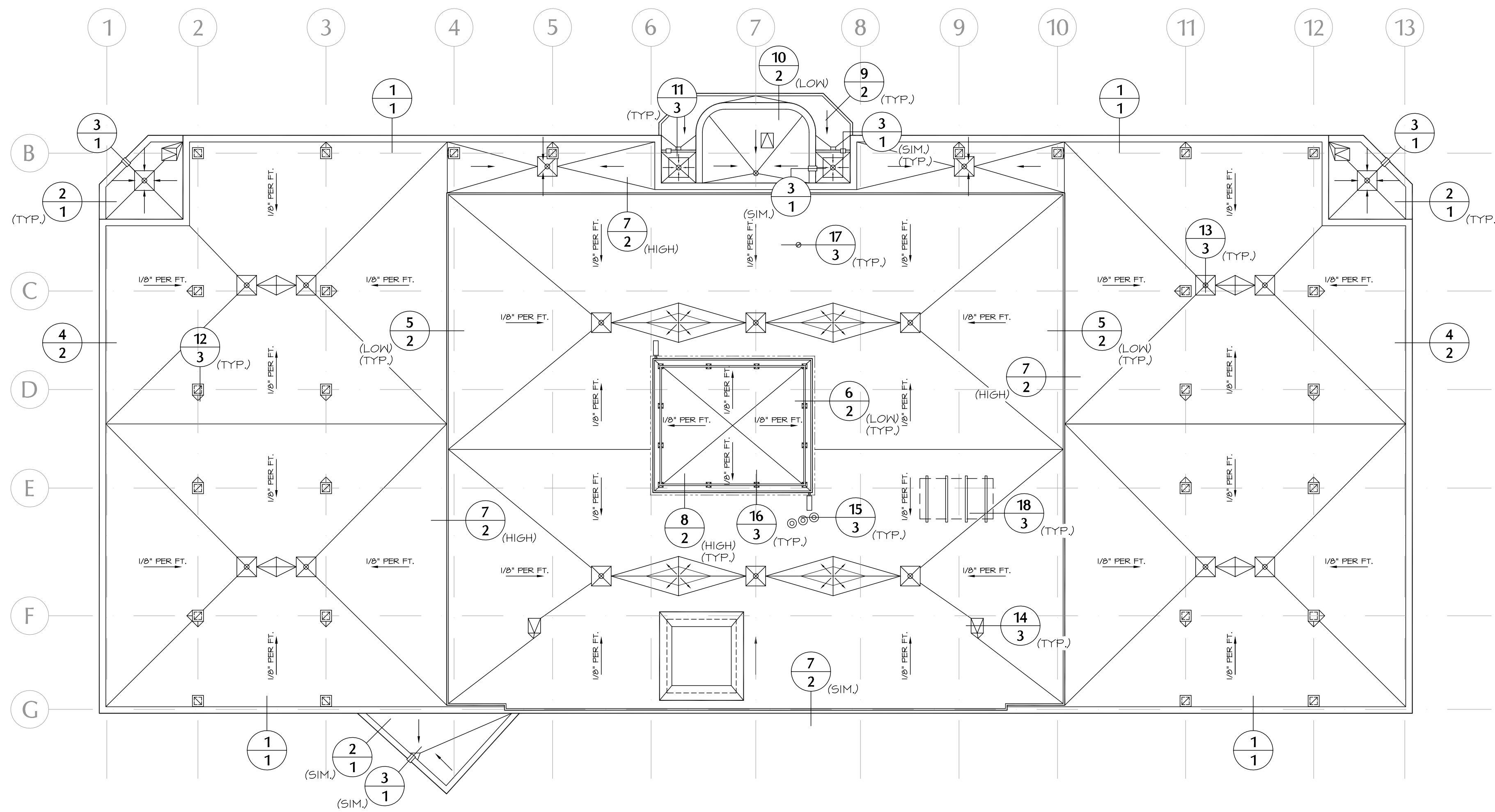
ROOF PLAN SCALE: 1/16"=1'-0"
