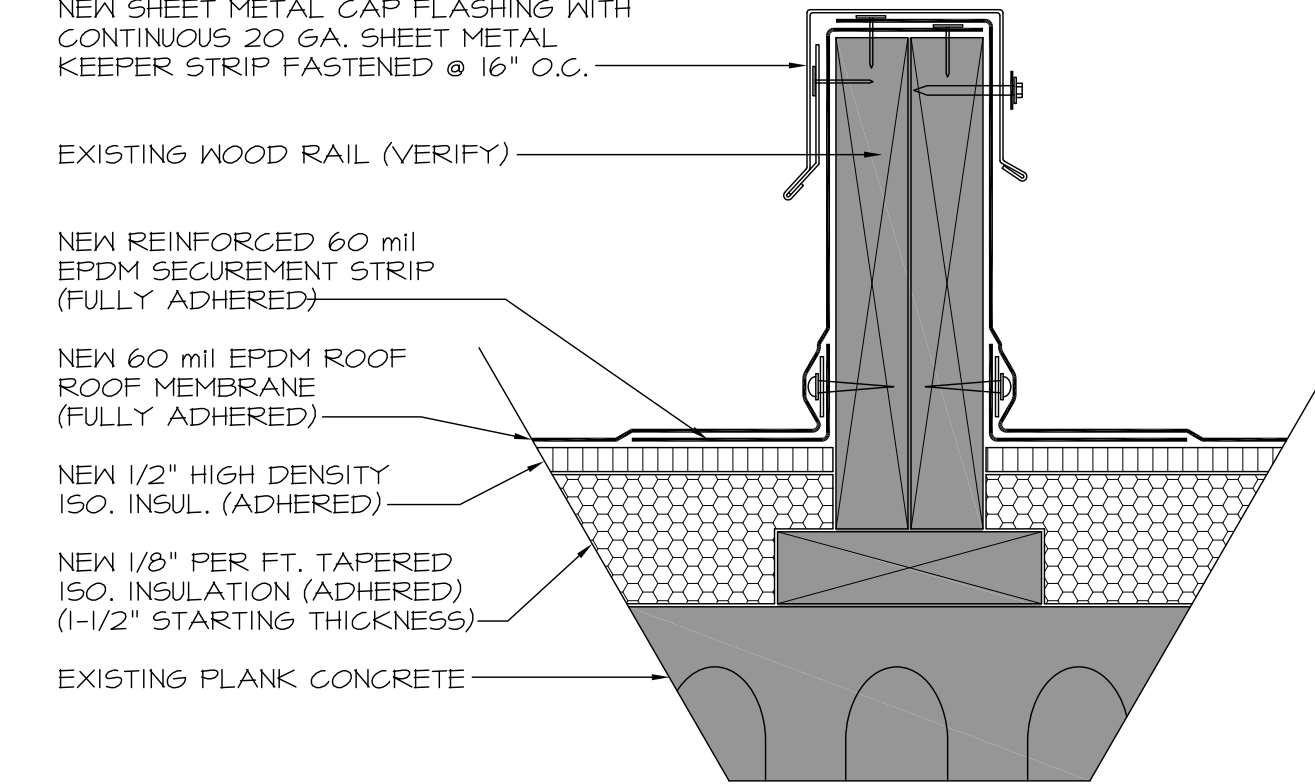
18 SOLAR PANEL SUPPORT DETAIL 3 SCALE: 3"=1'-0"
