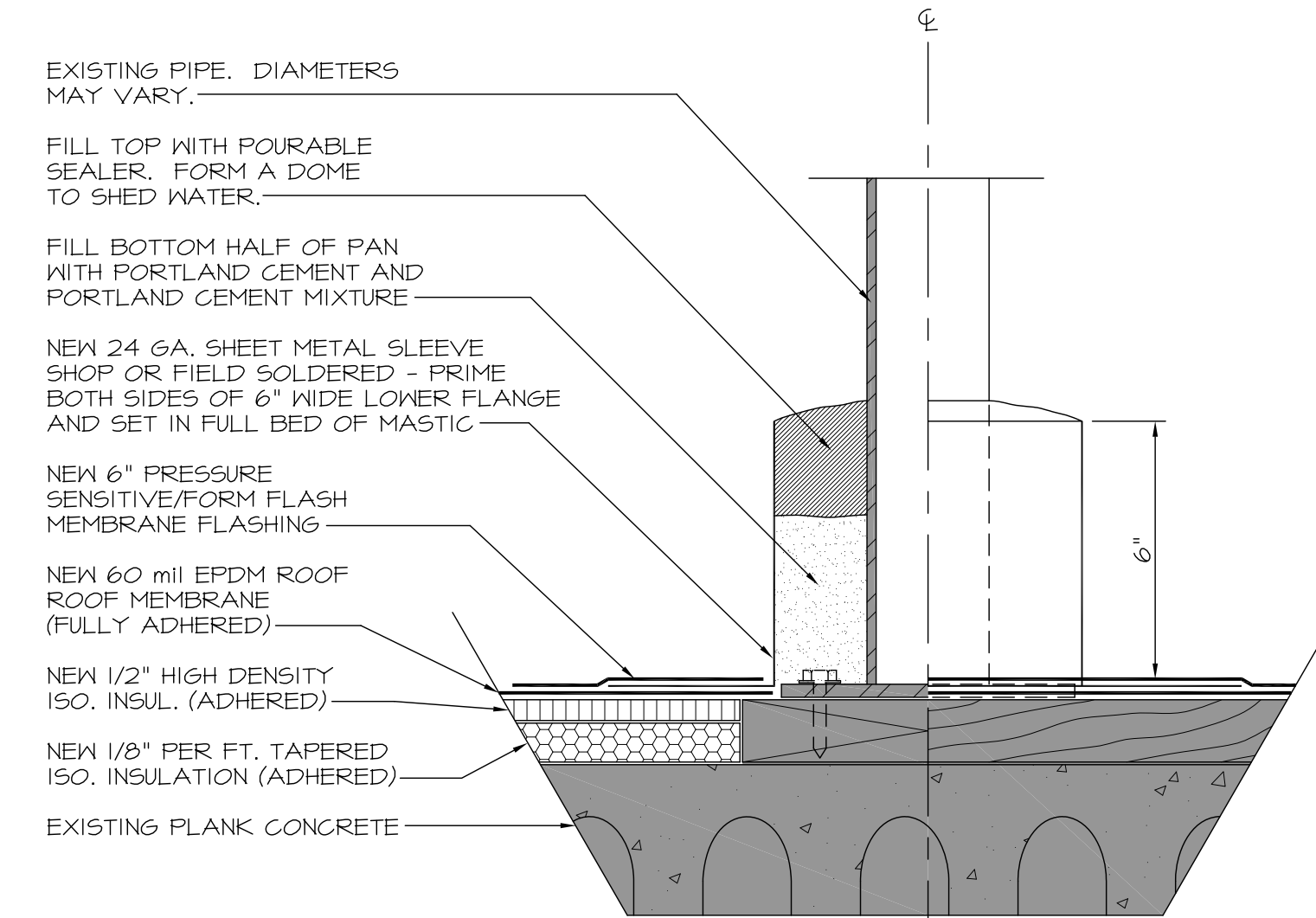
16 RAILING SUPPORT DETAIL 3 SCALE: 3"=1'-0"
