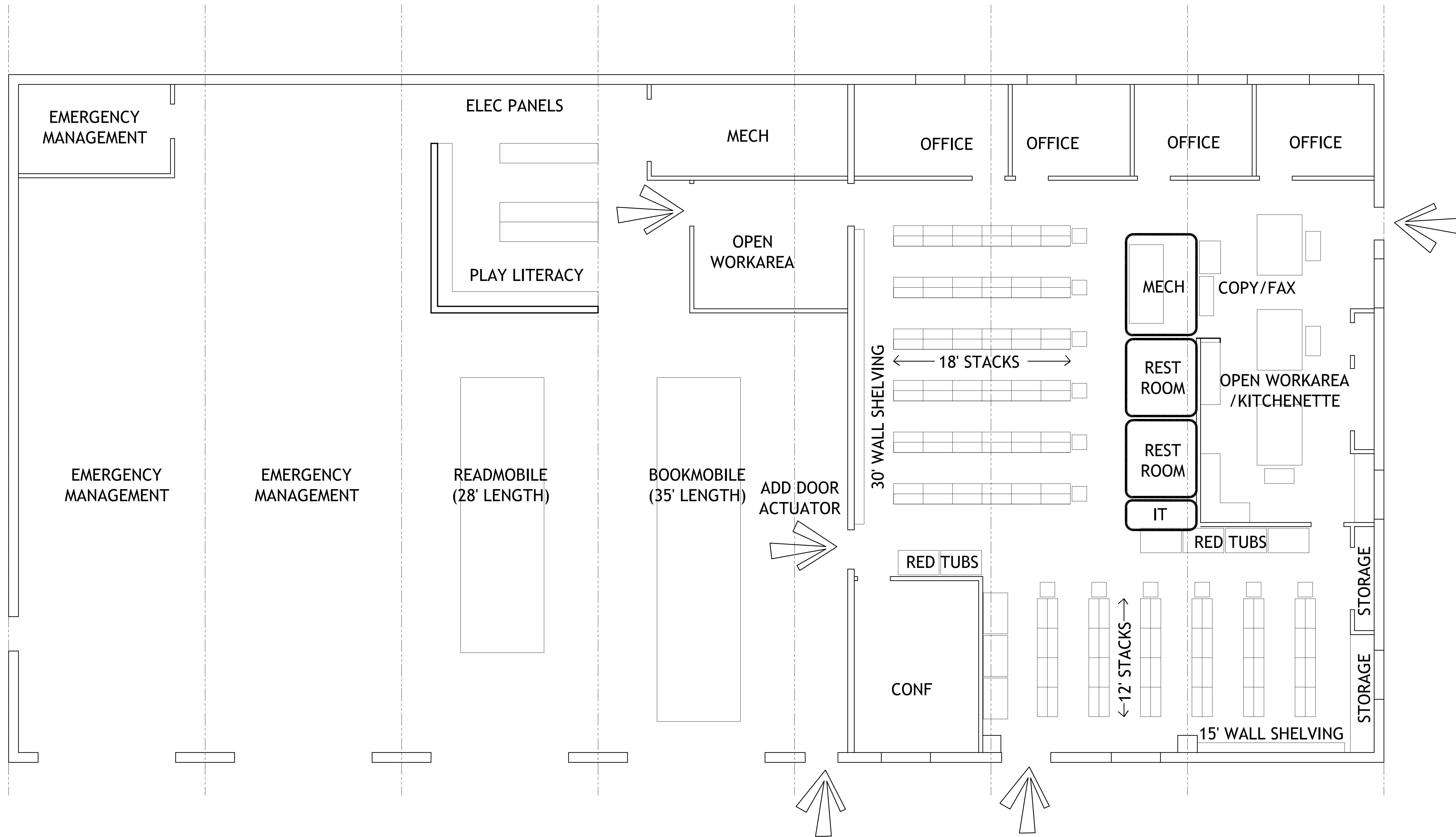
FIRST FLOOR CONCEPT FLOOR PLAN 08.24.16 3/16" = 1'-0"
