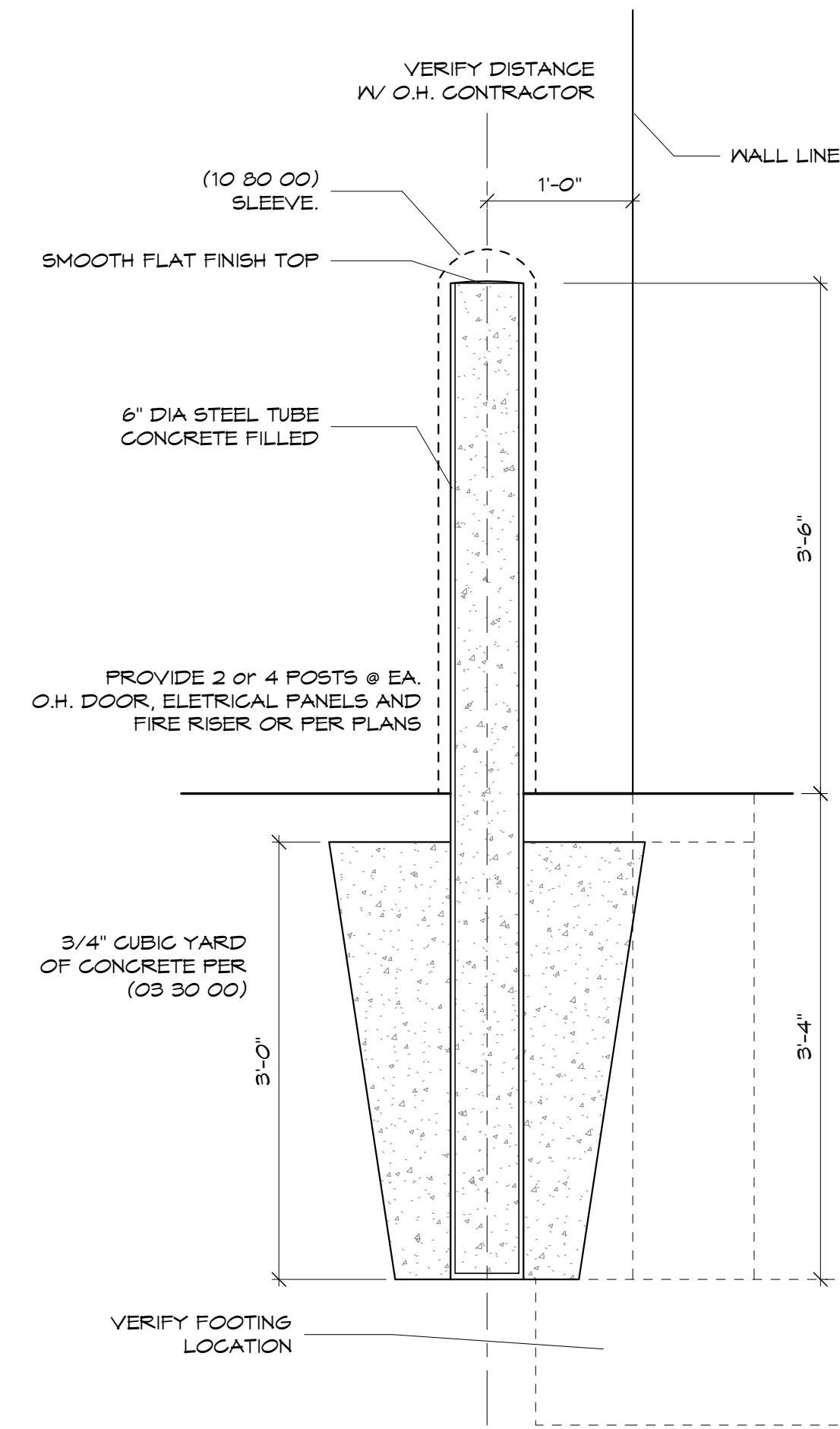
7 Concrete Bollard 1" = 1'-0"
