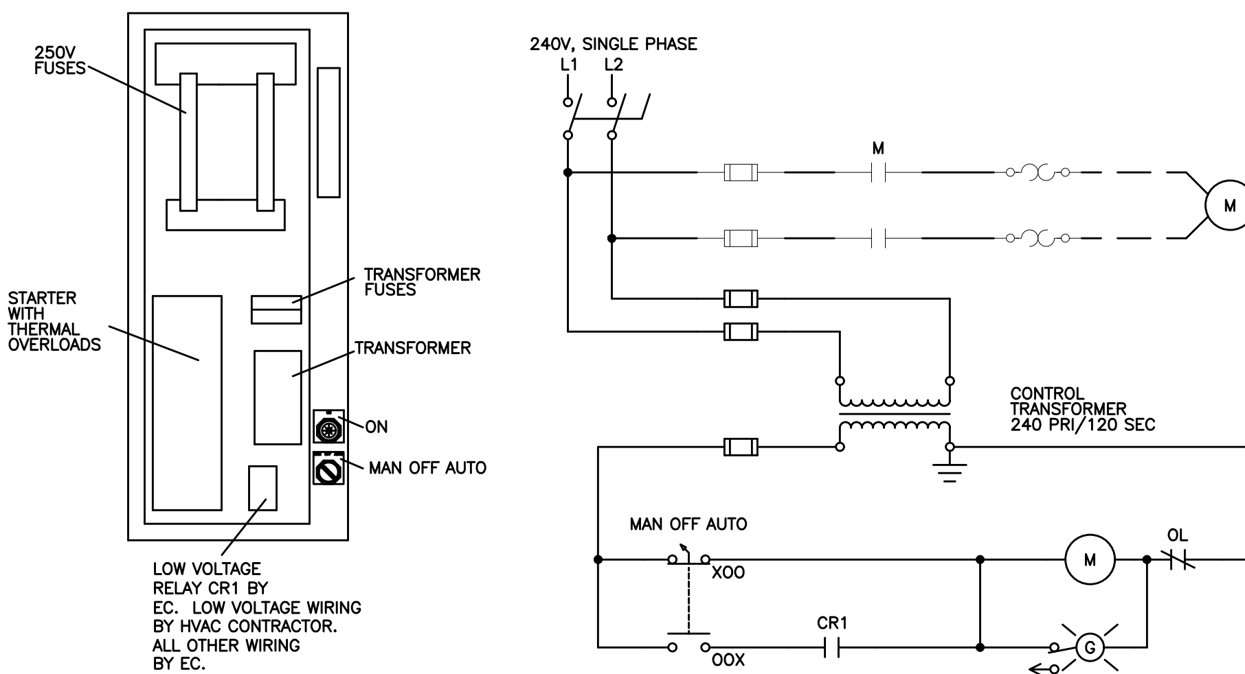
3 TYPICAL 240V SINGLE PHASE COMBINATION STARTER NO SCALE
