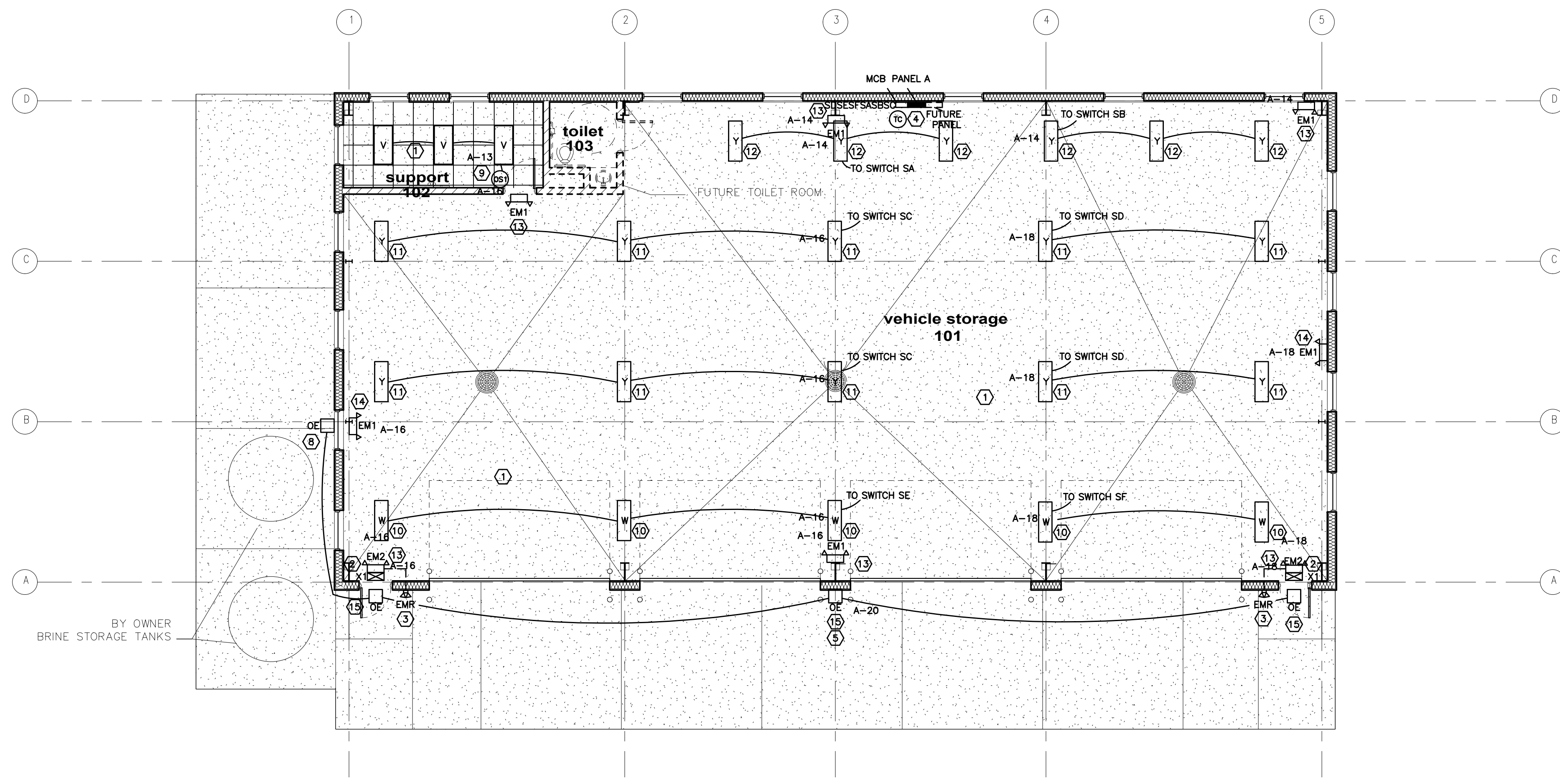
1 Satellite Building Lighting Plan 1/8" = 1'-0"
