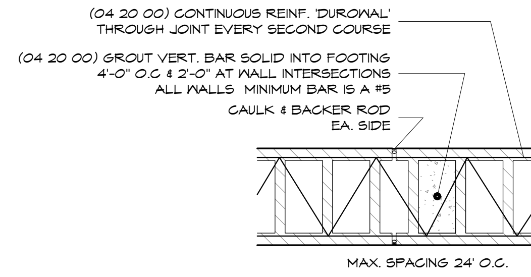
3 Masonry Control Joint 1 1/2" = 1'-0"
