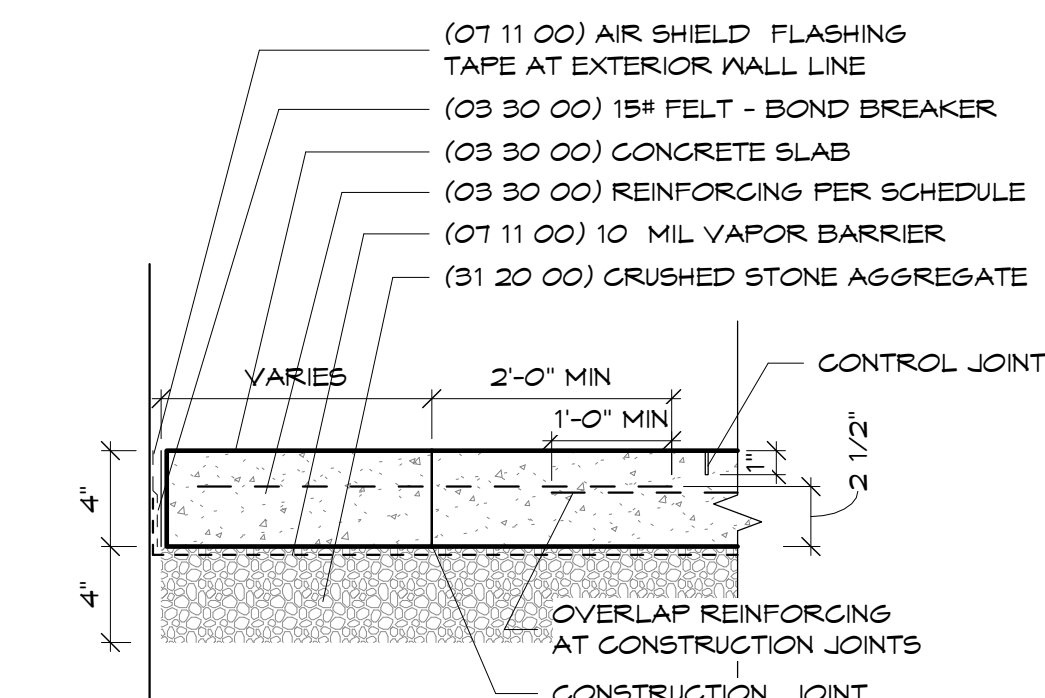
2 Concrete Slab - Type A 1 1/2" = 1'-0"
