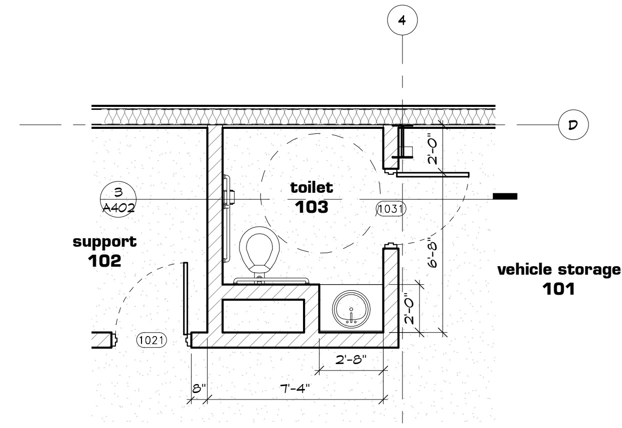
4 Future Enlarged Toilet Rooms 1/4" = 1'-0"
