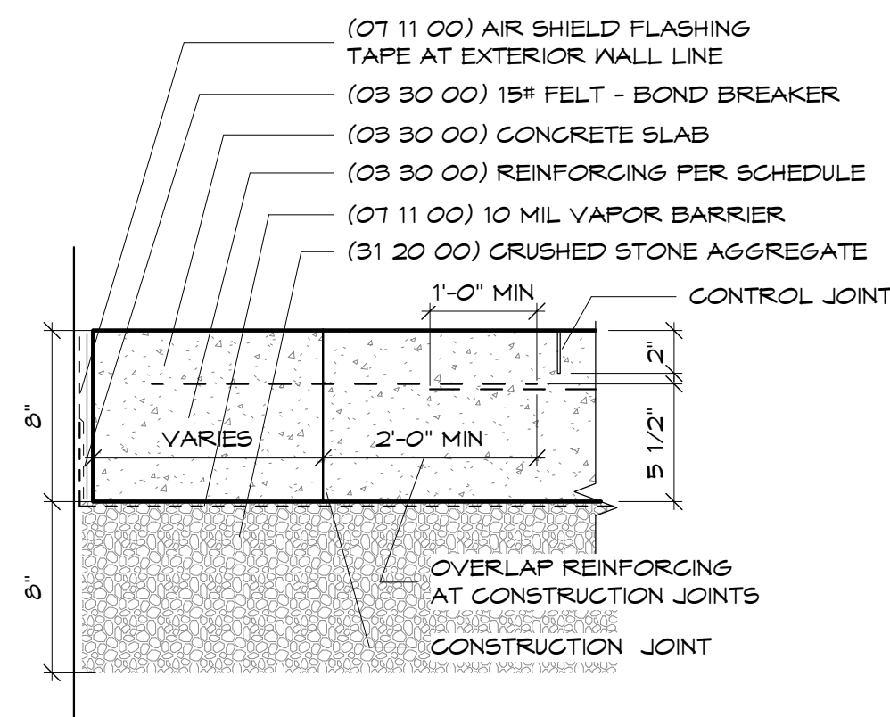
3 Concrete Slab - Type C 1 1/2" = 1'-0"
