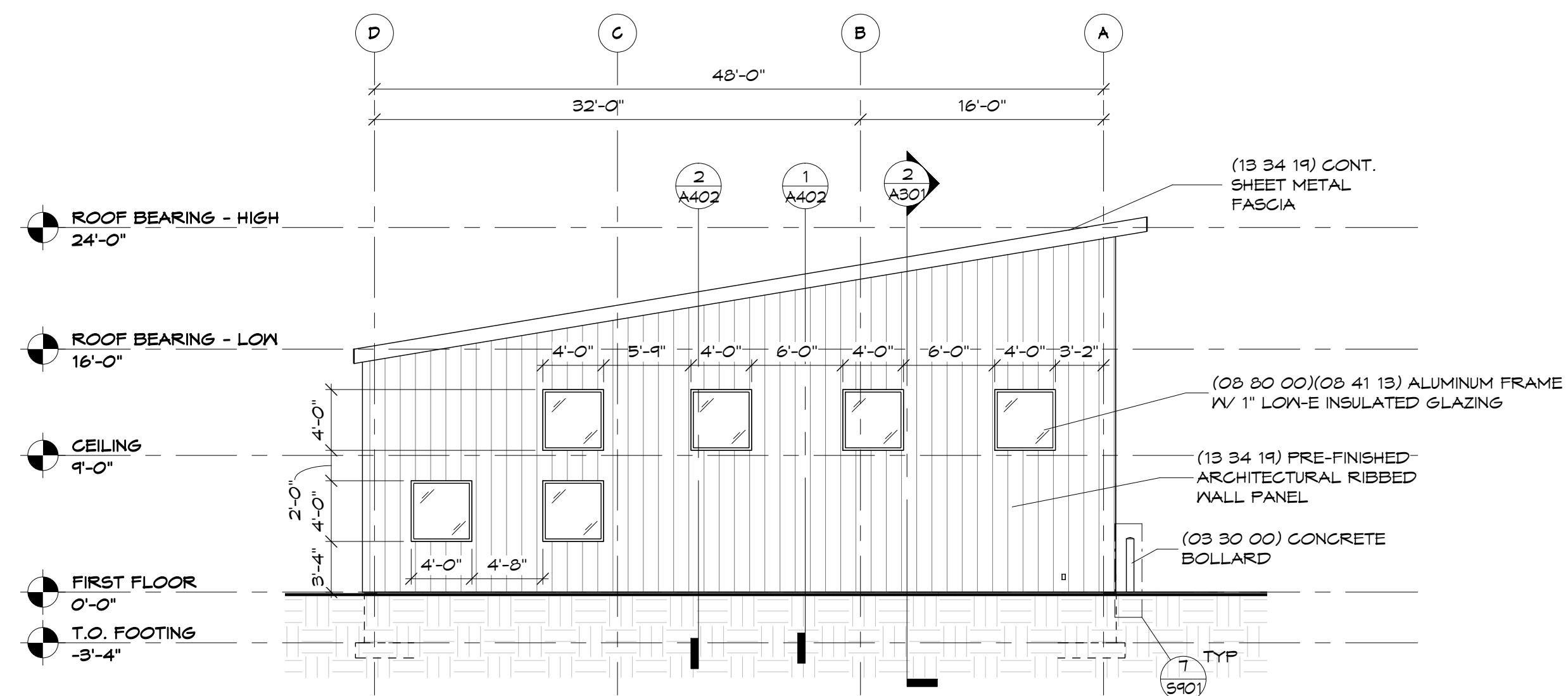
4 West Elevation 1/8" = 1'-0"
