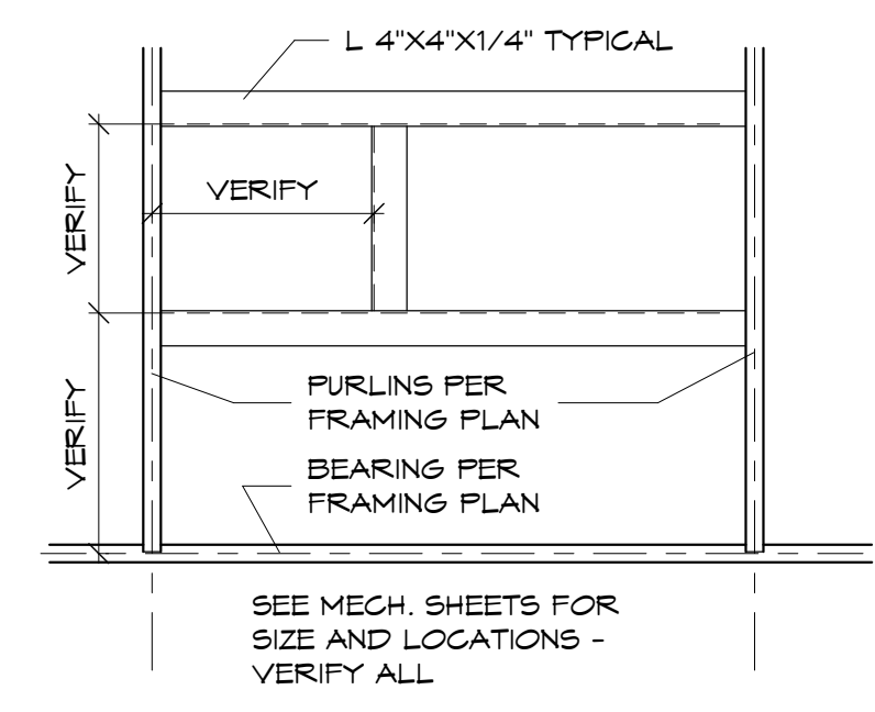
2 Framing at Roof Openings 1/2" = 1'-0"
