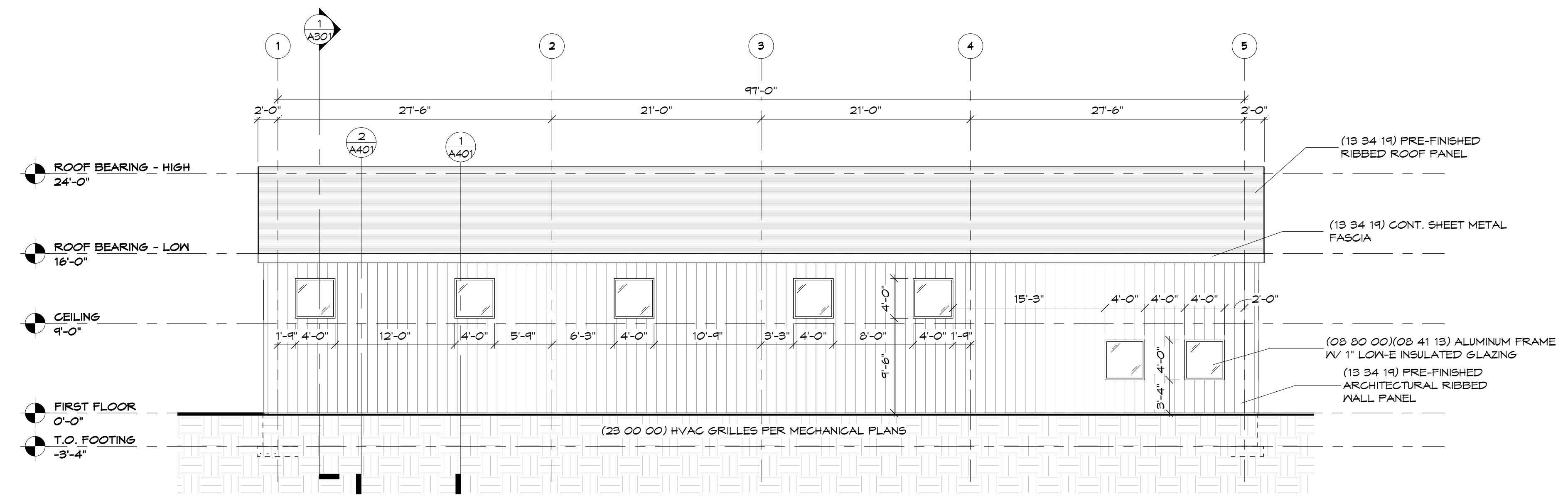
1 North Elevation 1/8" = 1'-0"
