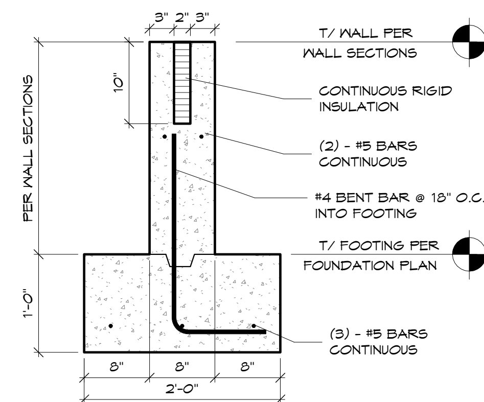
4 Foundation Wall and Footing - Typ 1" = 1'-0"
