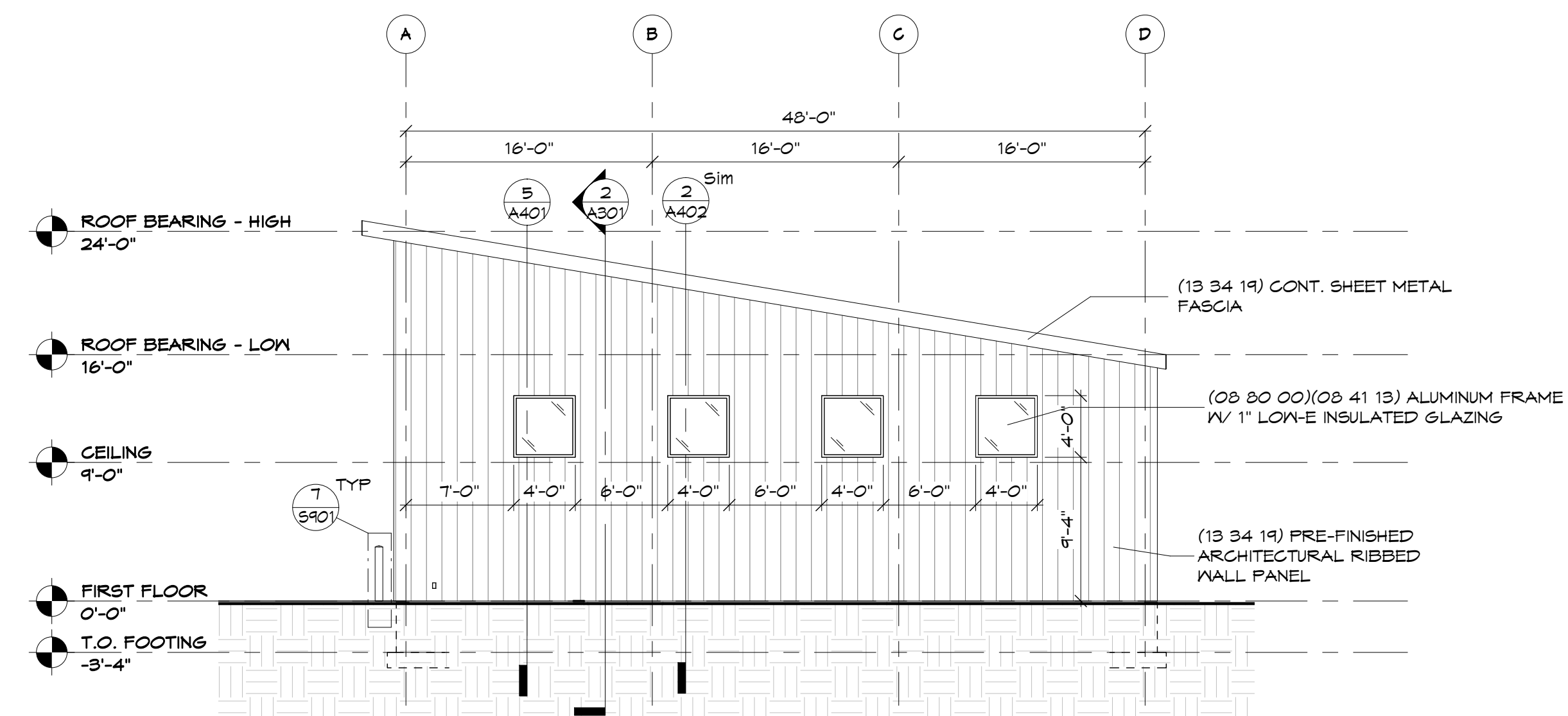
2 East Elevation 1/8" = 1'-0"
