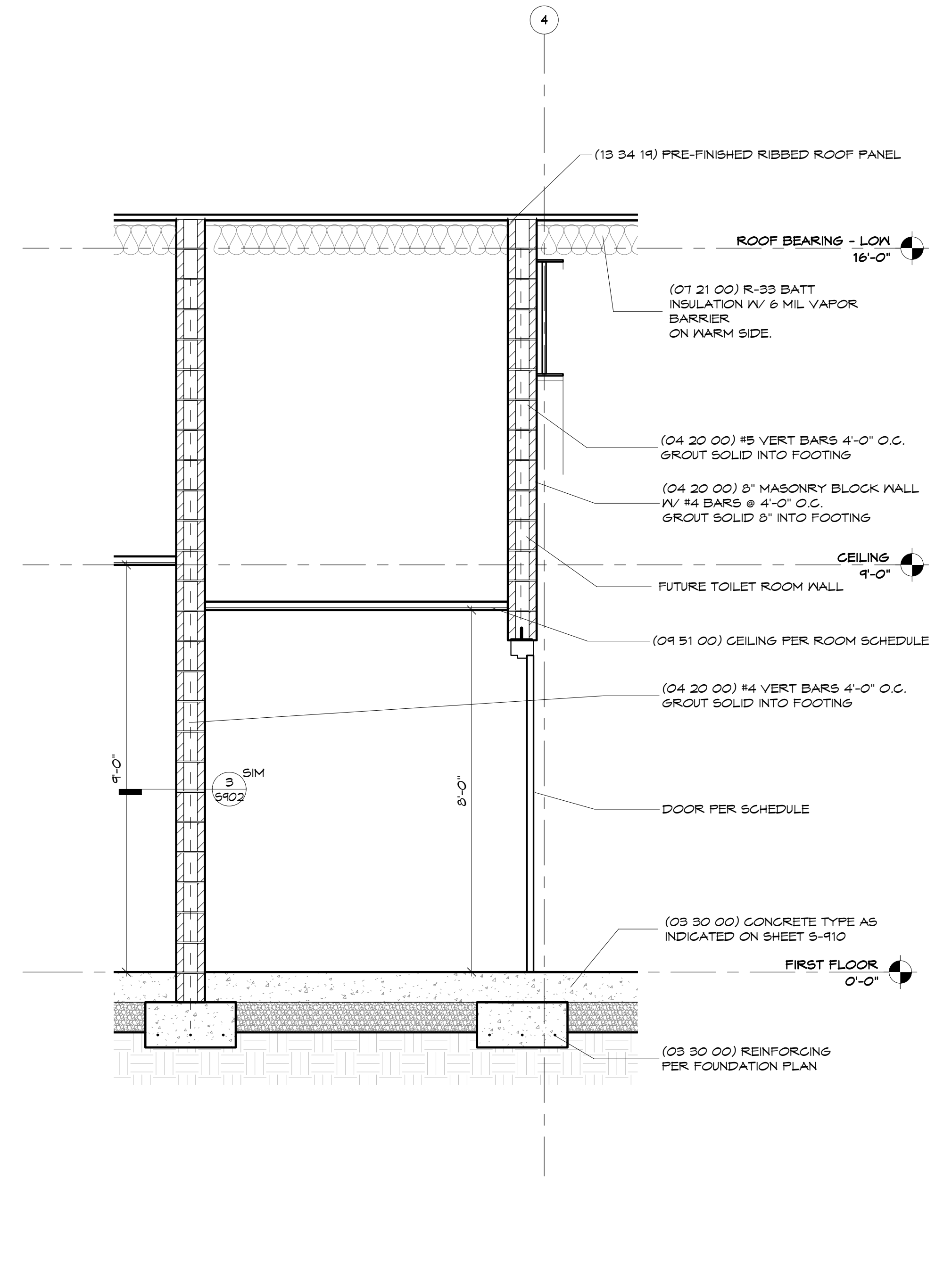
3 Wall Section 1/2" = 1'-0"
