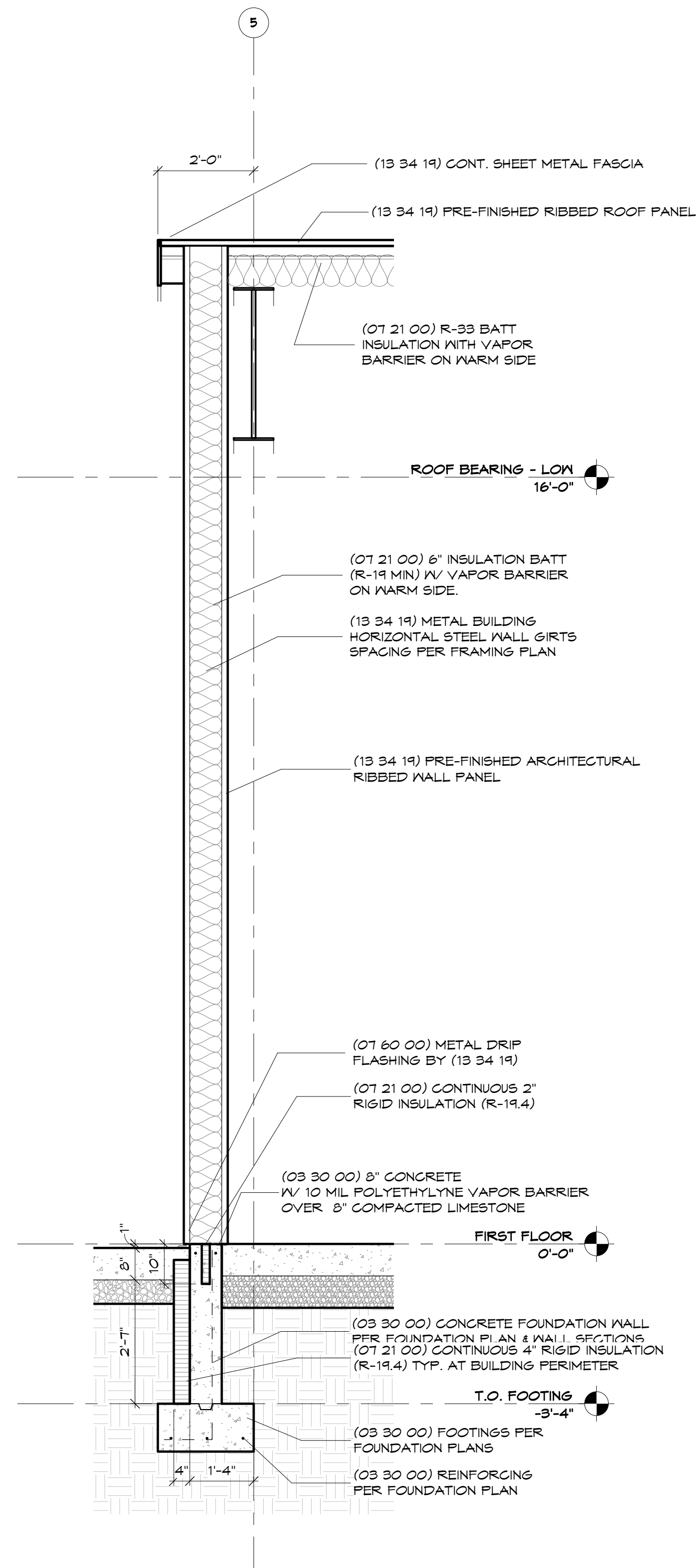
1 Wall Section 1/2" = 1'-0"
