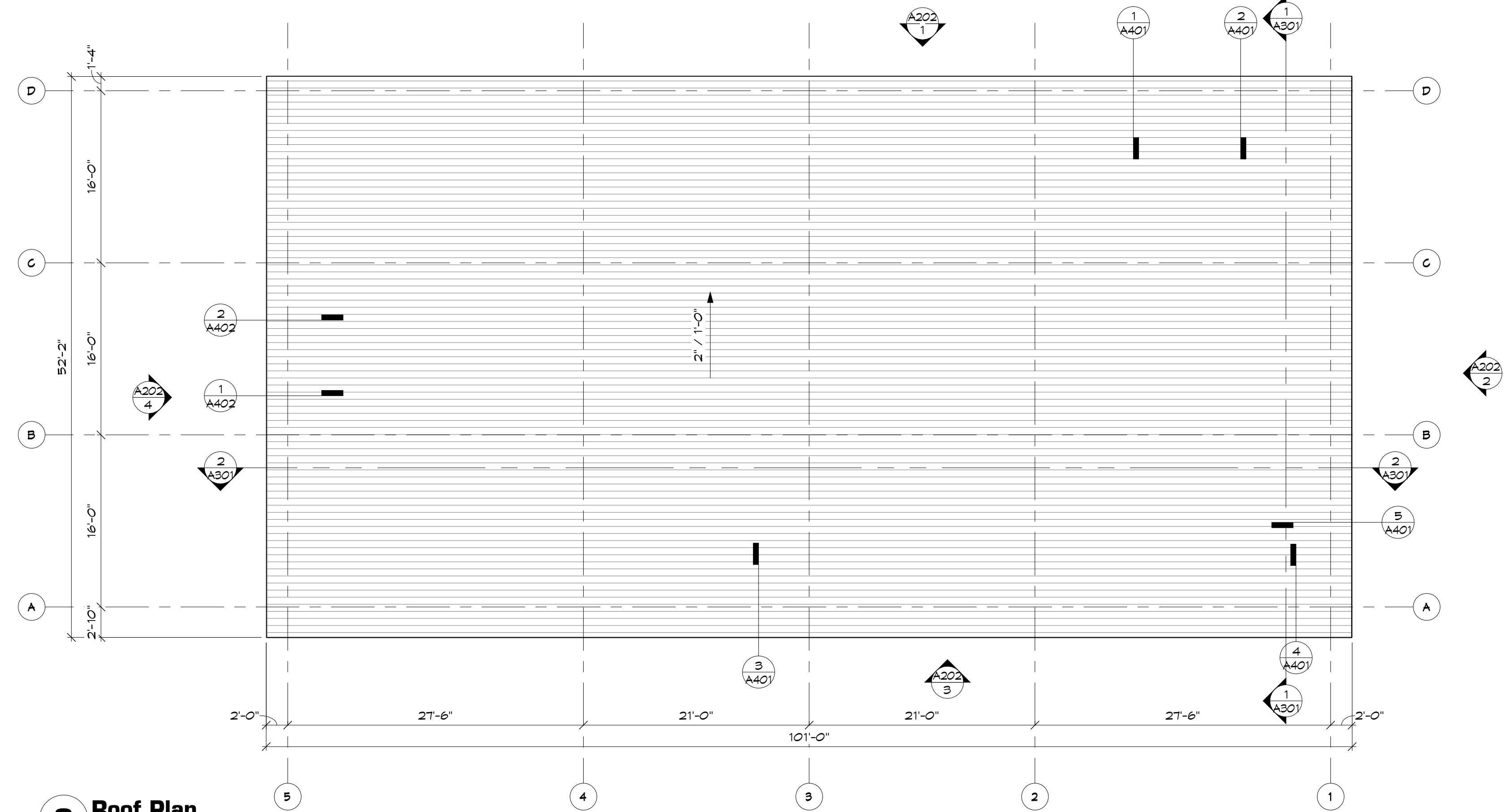
2 Roof Plan 1/8" = 1'-0"
