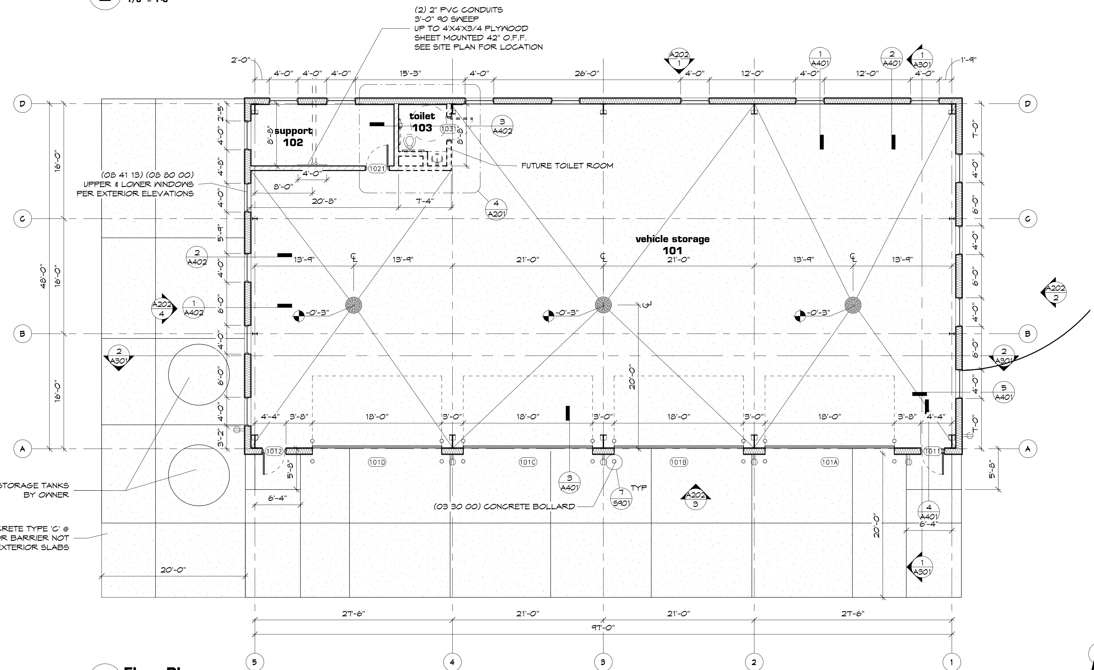
1 Floor Plan 1/8" = 1'-0"
