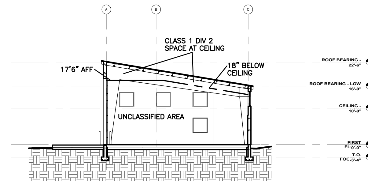
2 CNG CLASSIFIED CEILING SPACE
