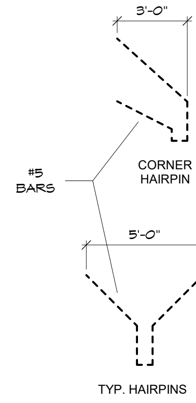
6 Typ. Hairpins 1/4" = 1'-0"
