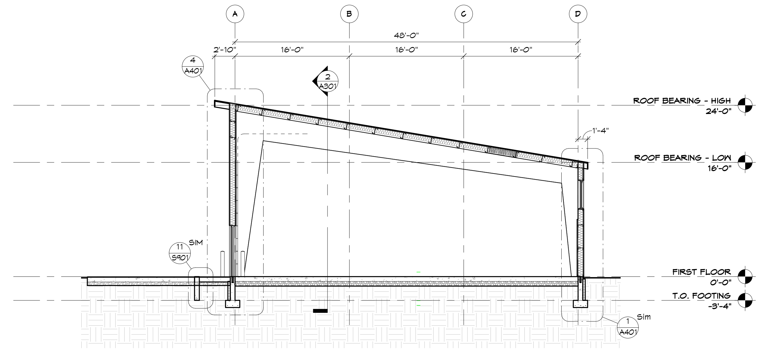
1 EW Building Section 1/8" = 1'-0"
