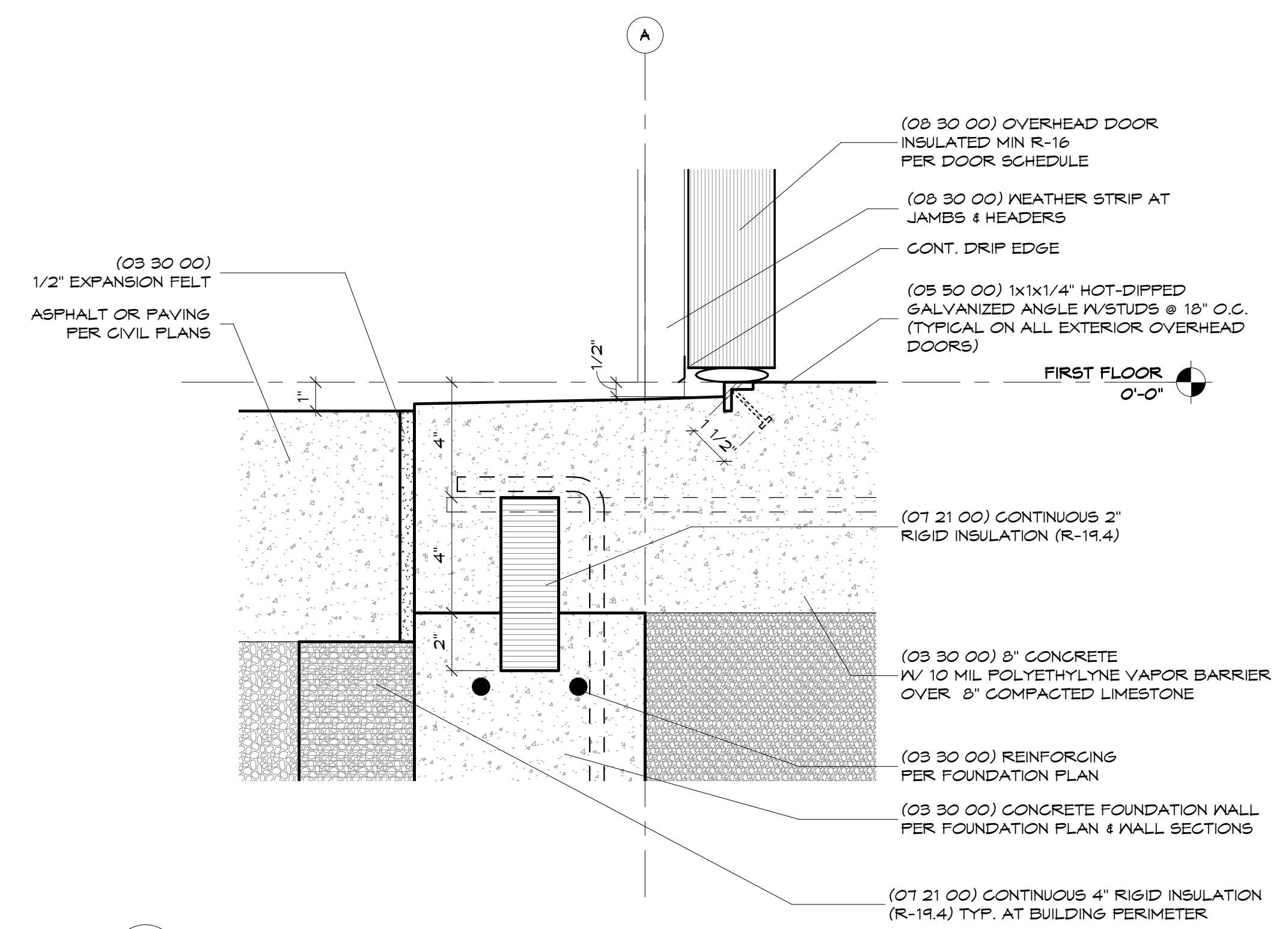
5 OH Door Threshold 3" = 1'-0"
