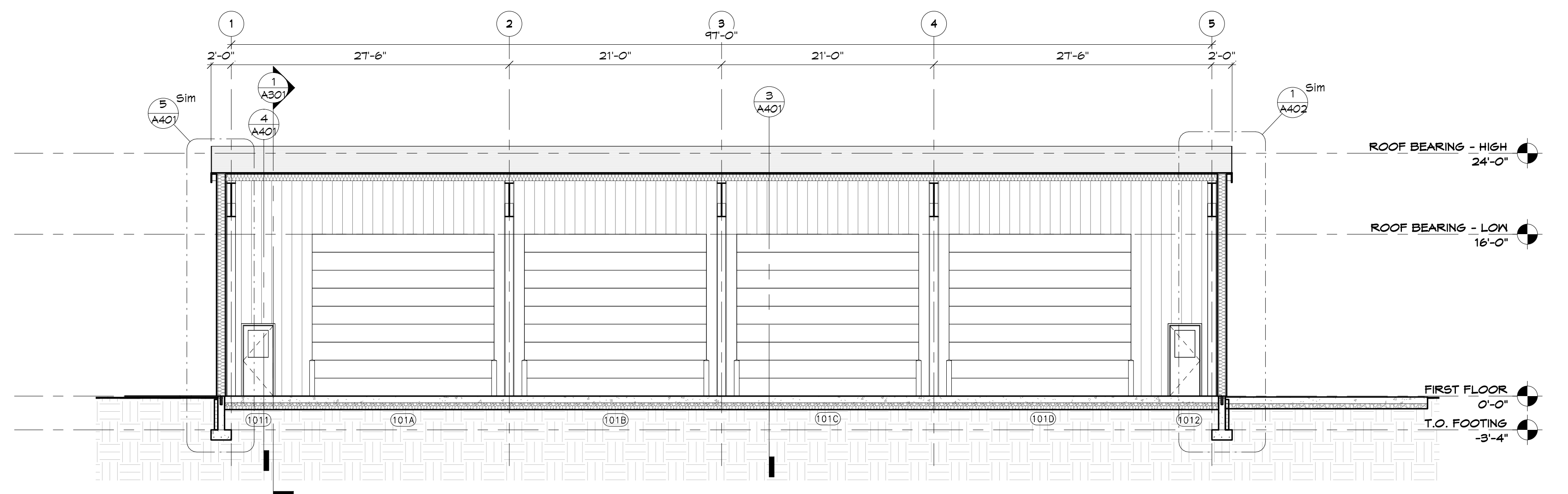
2 North-South Building Section 1/8" = 1'-0"
