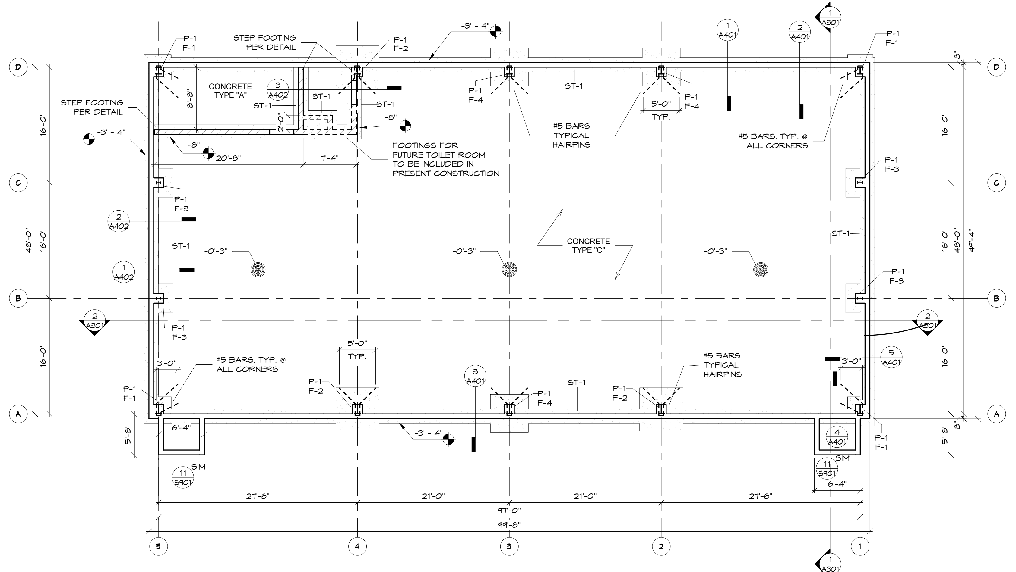
1 Foundation Plan 1/8" = 1'-0"
