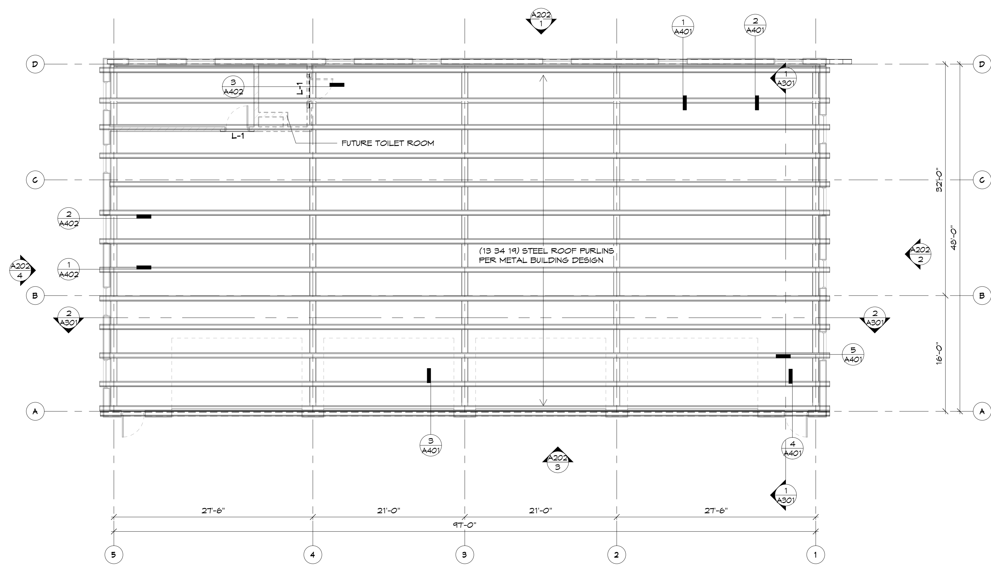
1 Roof Framing Plan 1/8" = 1'-0"
