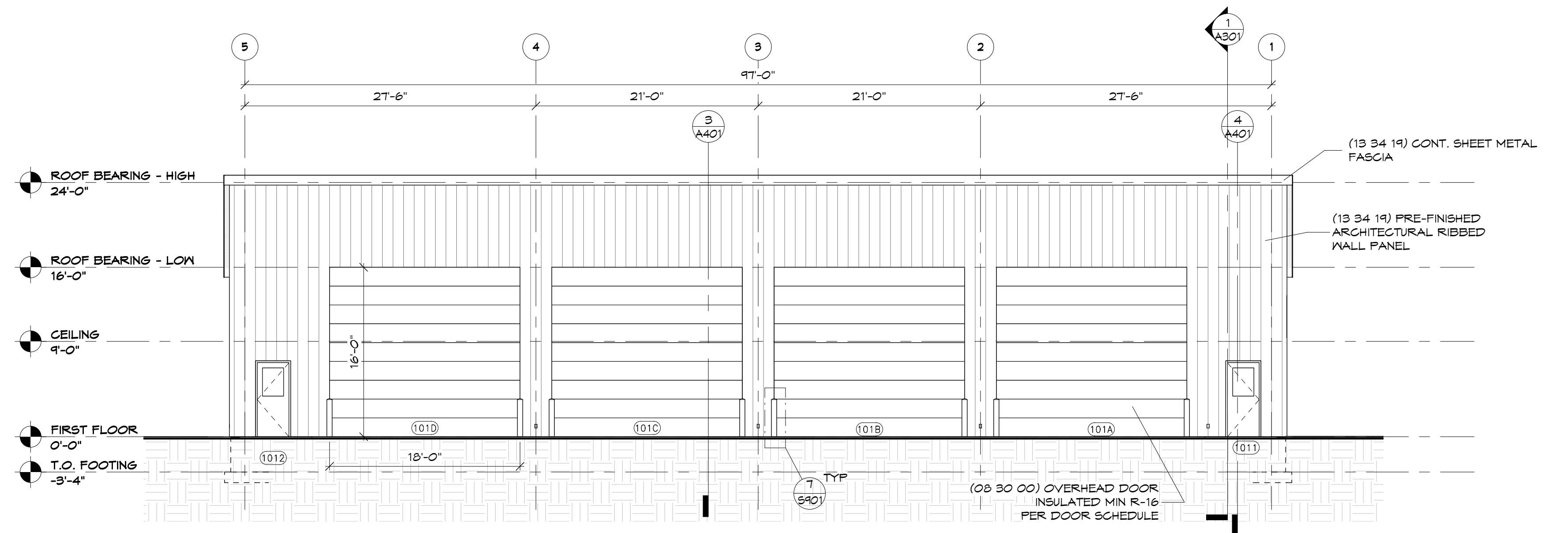
3 South Elevation 1/8" = 1'-0"
