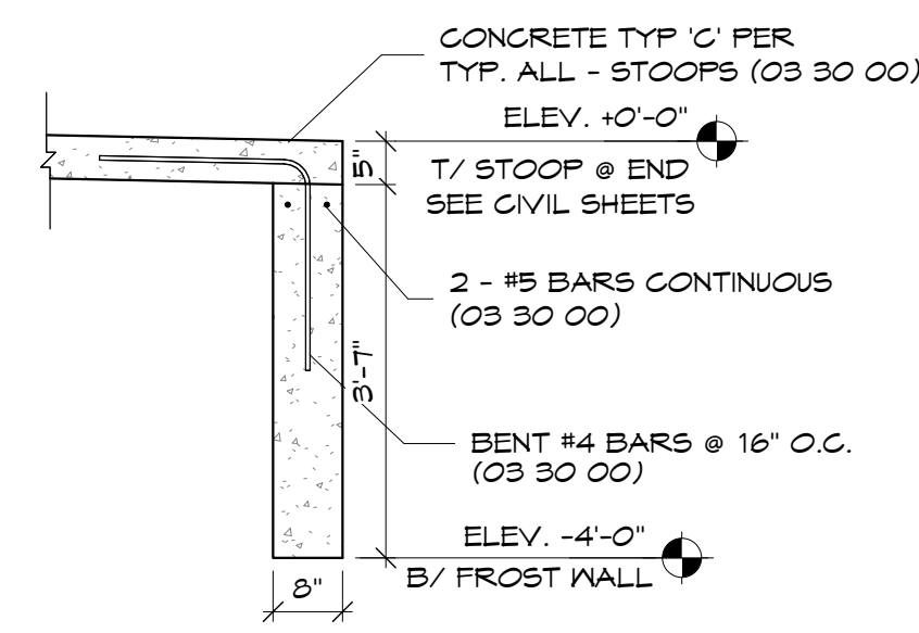
11 Stoop Frost Wall 1/2" = 1'-0"
