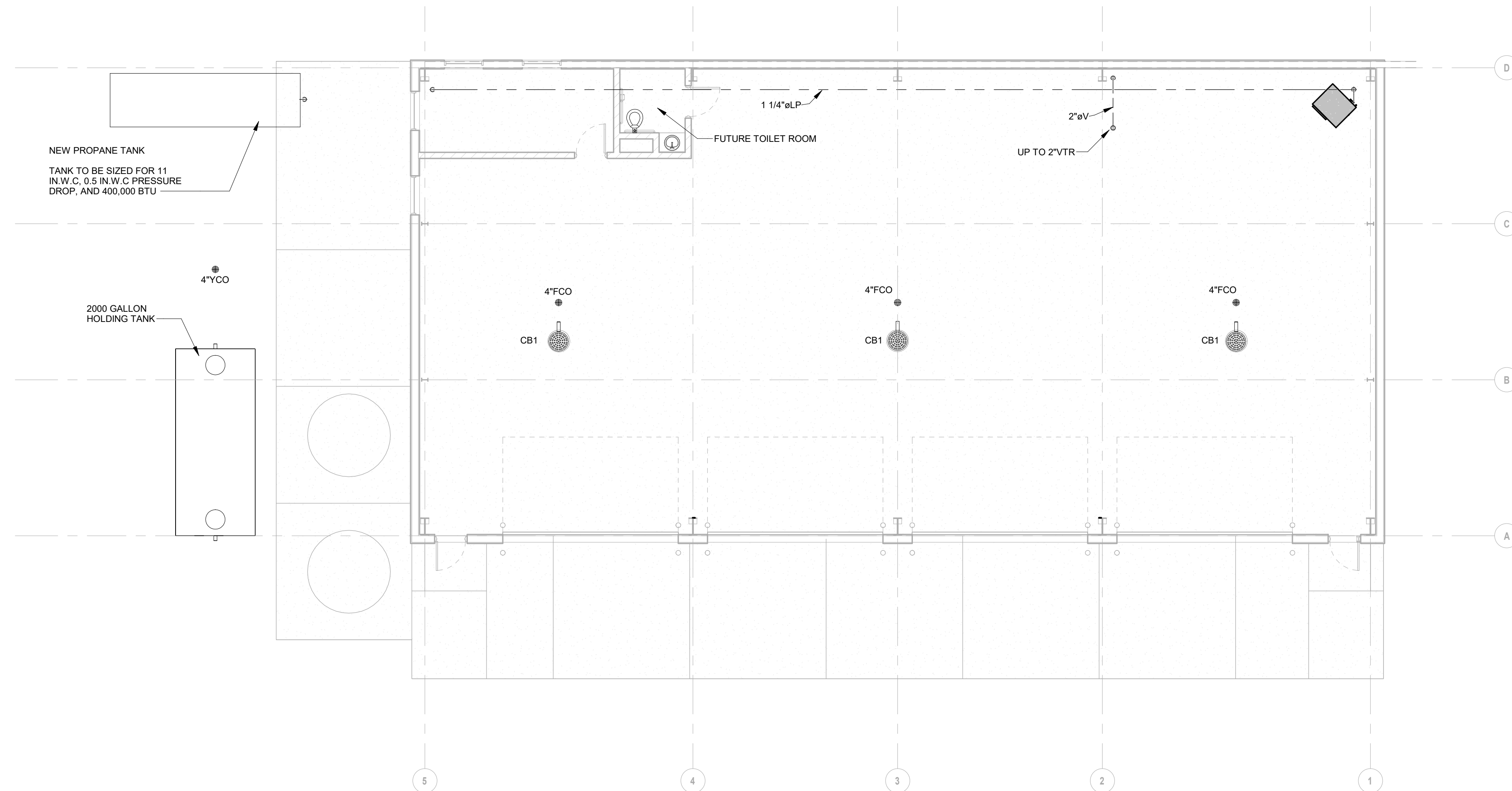
1 Above Ground Plumbing Plan P100 SCALE: 1/8" = 1'-0"
