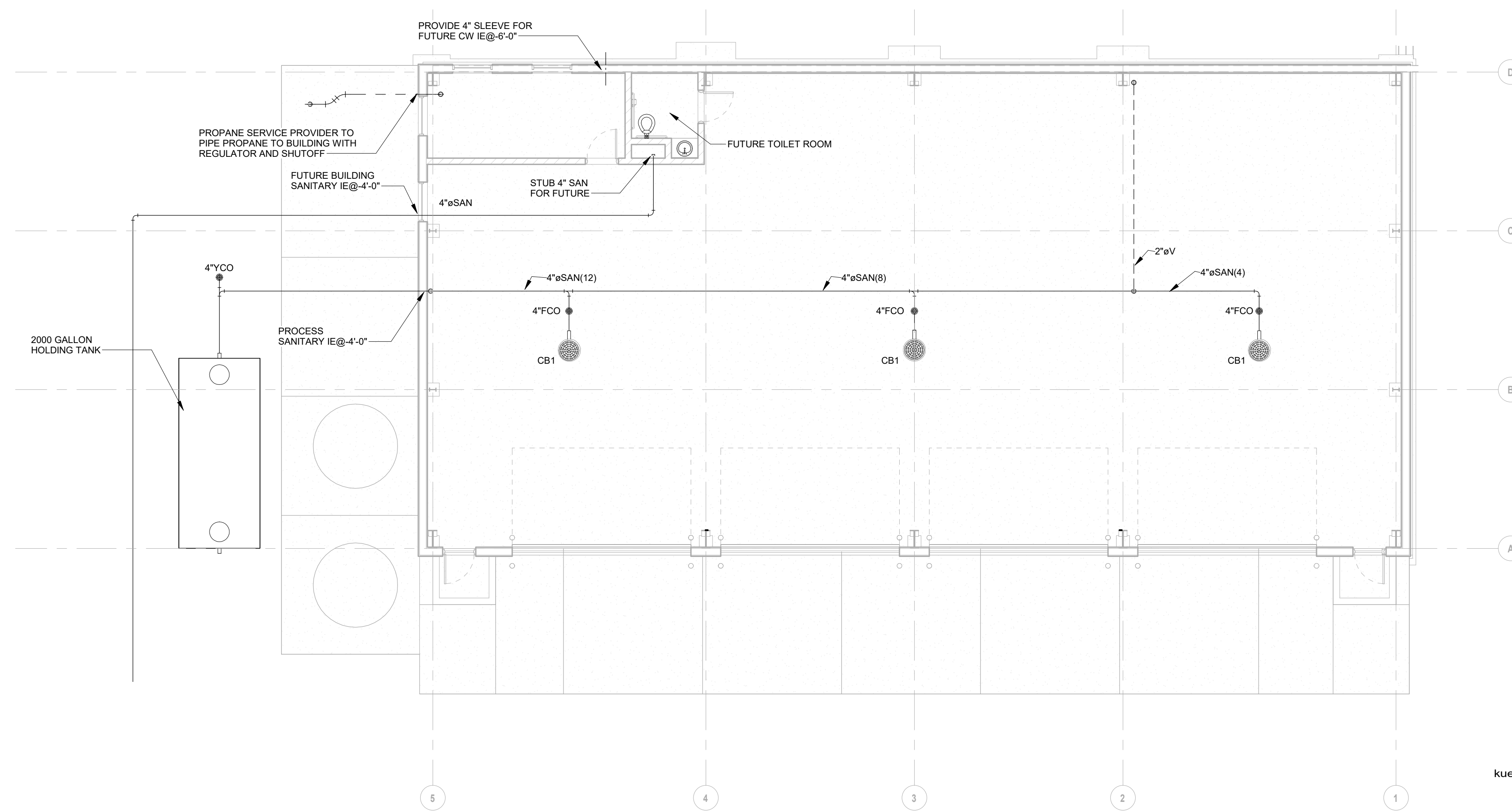
2 Underground Plumbing Plan P100 SCALE: 1/8" = 1'-0"
