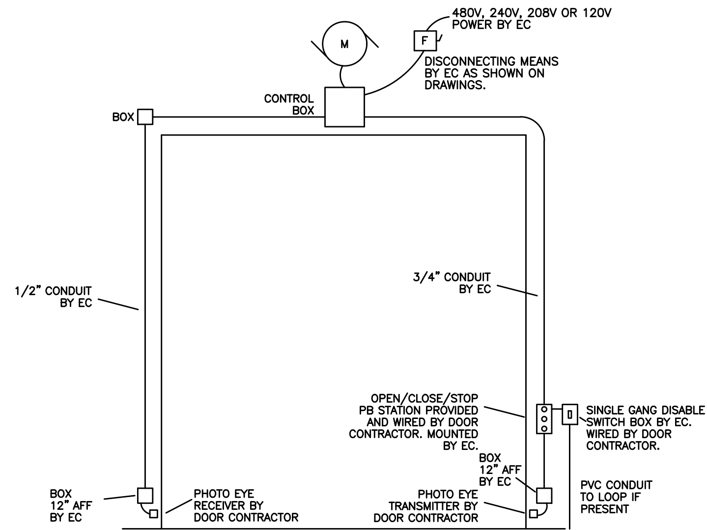
1 TYPICAL: OVERHEAD DOOR
