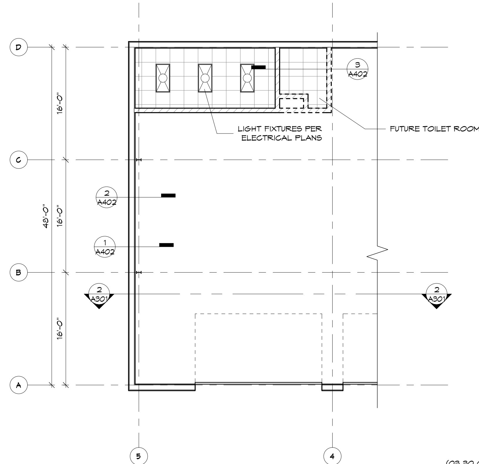
3 Reflected Ceiling Plan 1/8" = 1'-0"
