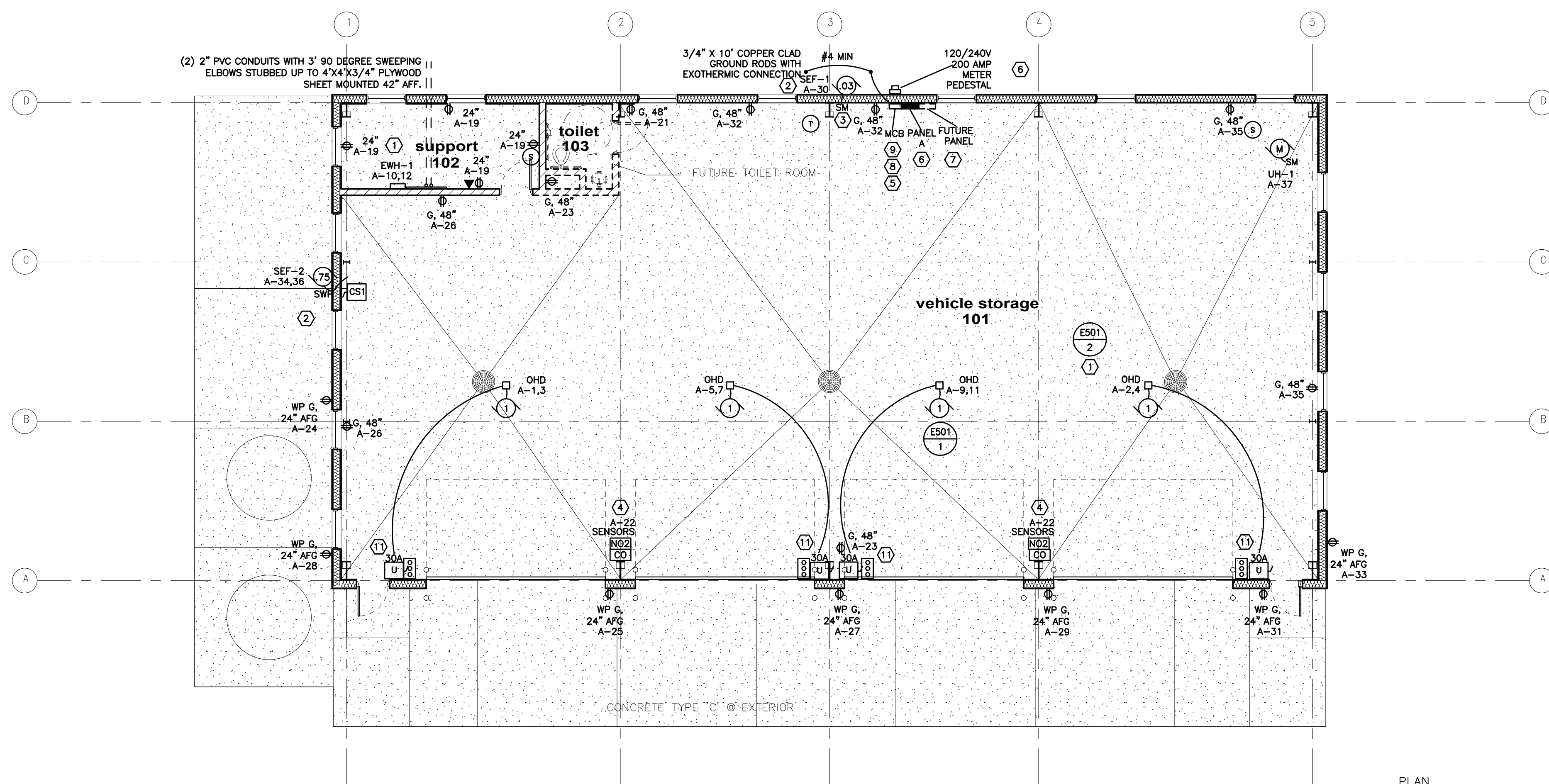
2 Satellite Building Power and Systems Plan 1/8" = 1'-0"
