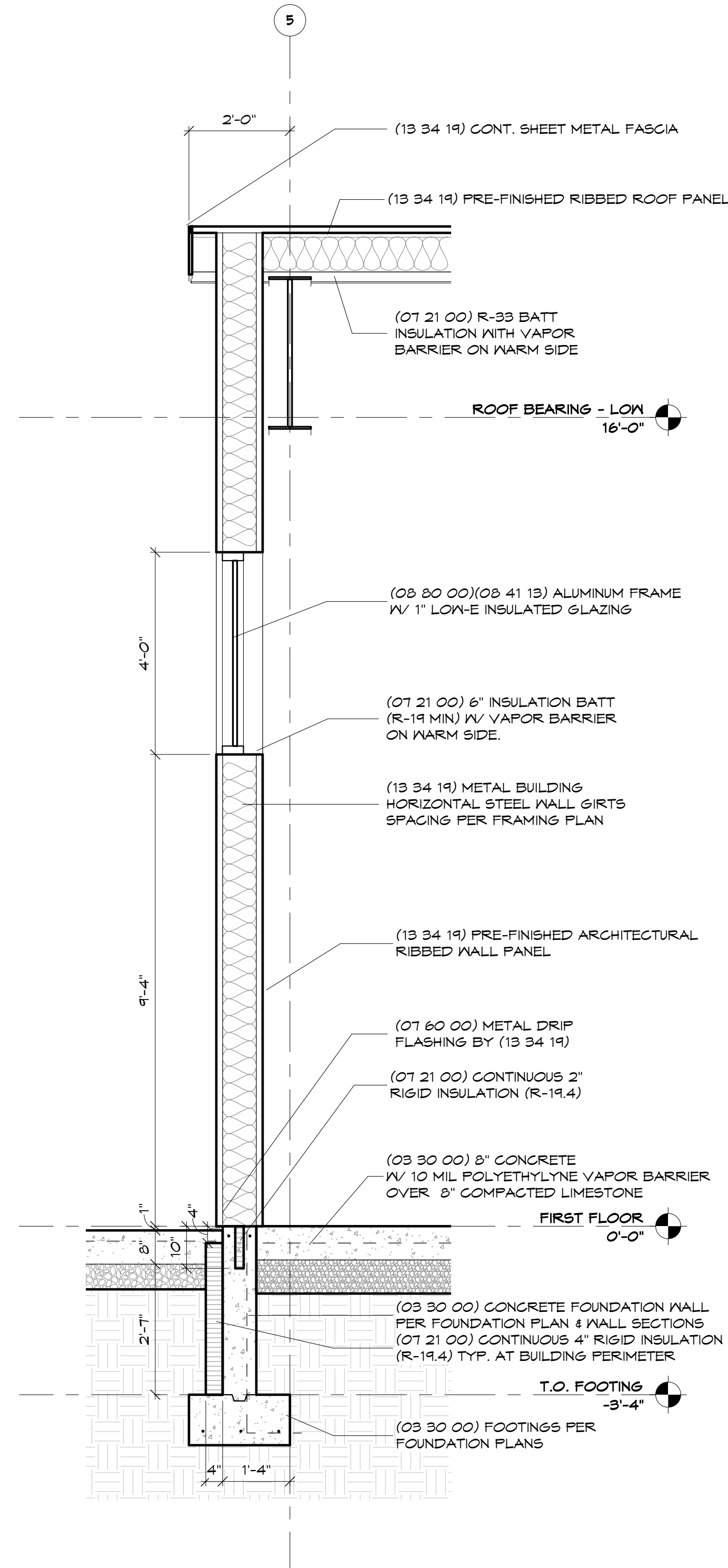
2 Wall Section 1/2" = 1'-0"
