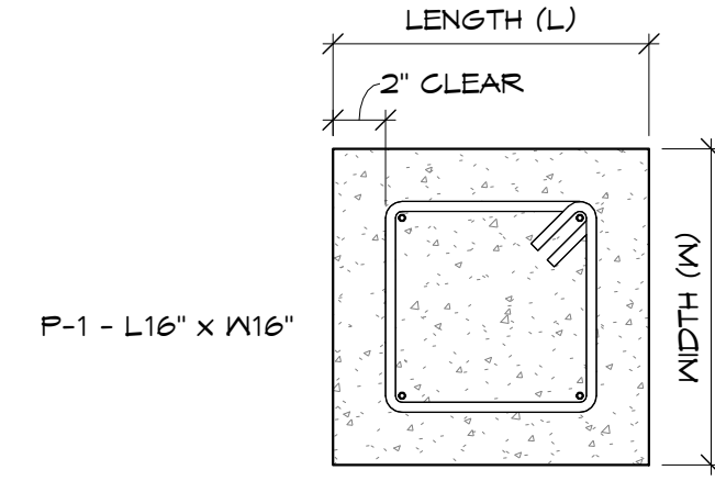
10 Pier Reinforcing Detail 1 1/2" = 1'-0"
