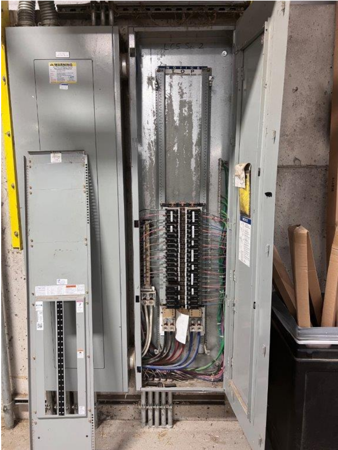
Panel LC5 (shown on sheet E203)
