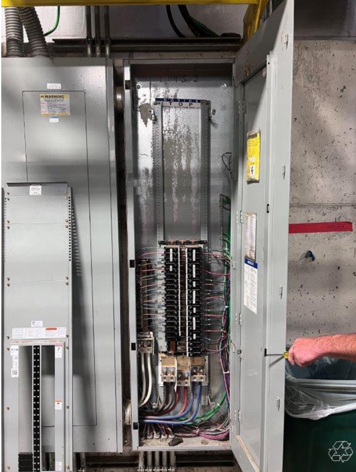
Panel LC4 (shown on sheet E203)
