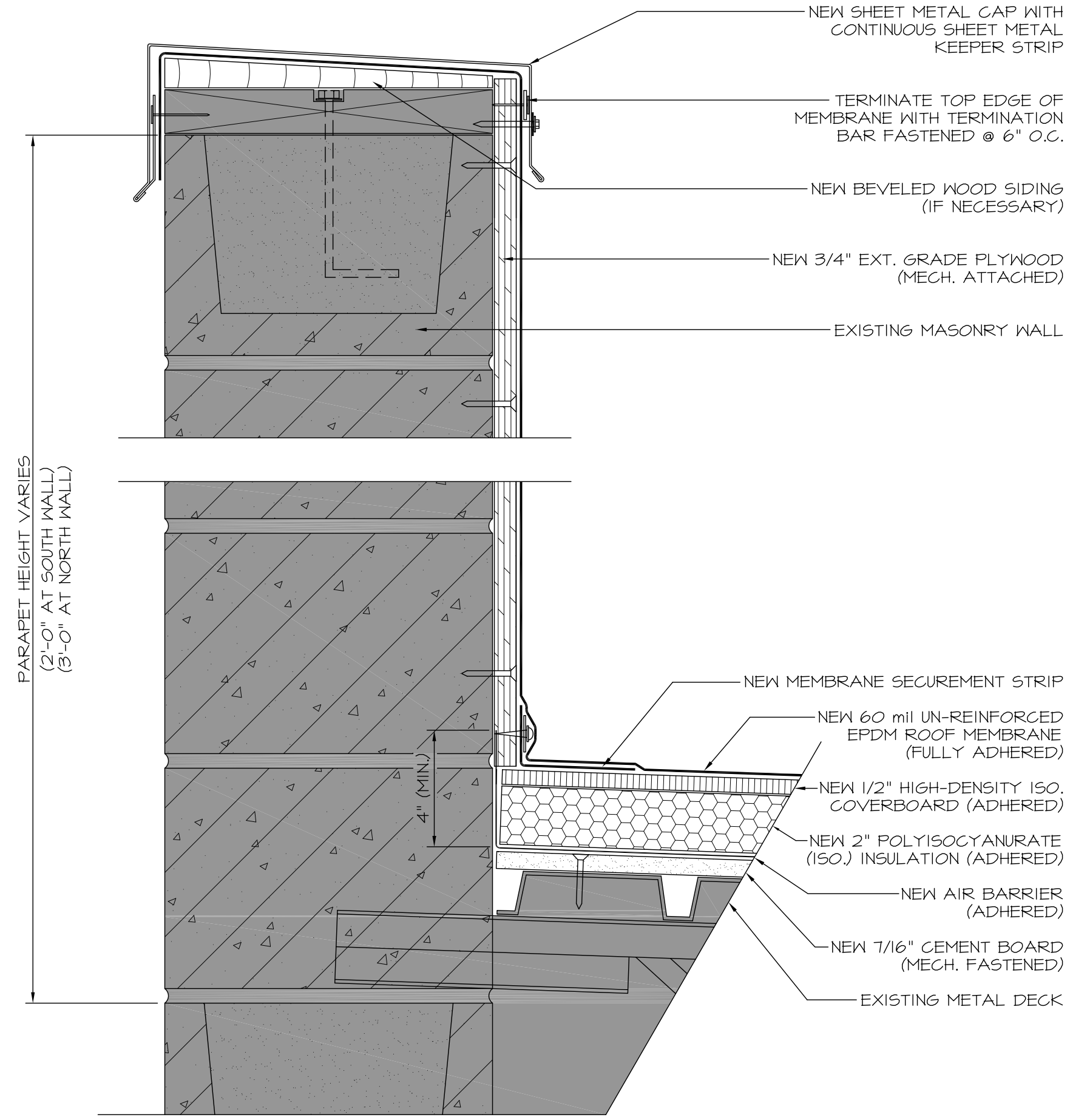
1 PARAPET FLASHING DETAIL SCALE: 3/8"=1'-0"
