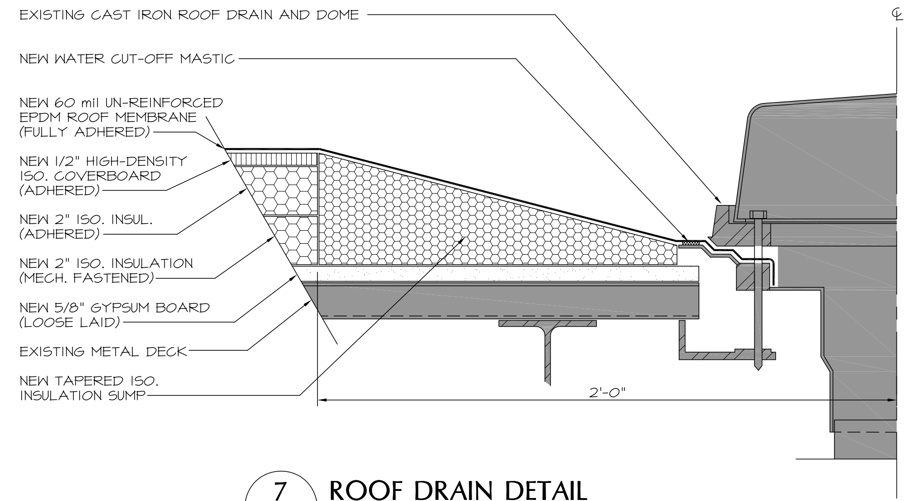
7 ROOF DRAIN DETAIL 2 SCALE: 3"=1'-0" TYPICAL
