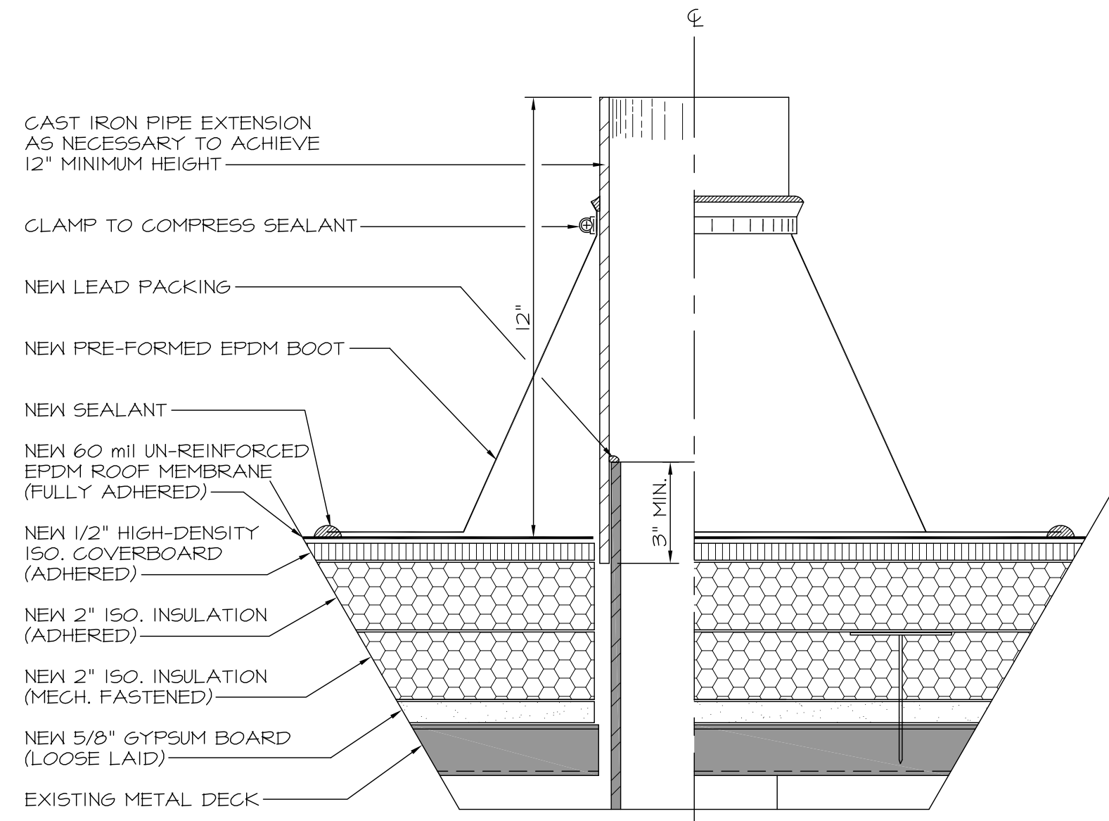
5 PLUMBING VENT DETAIL 2 SCALE: 3"=1'-0" TYPICAL
