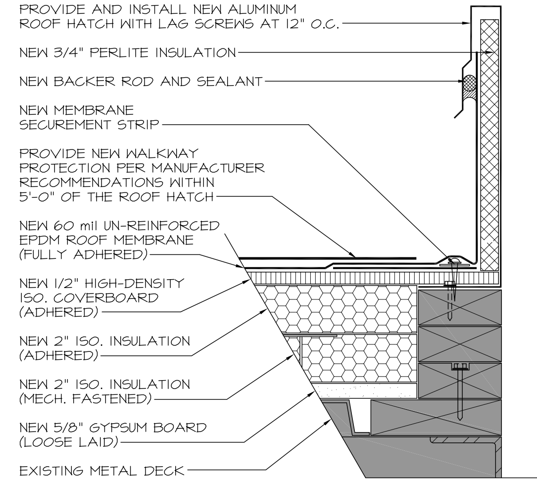
6 ROOF SCUTTLE DETAIL 2 SCALE: 3"=1'-0" AREA A
