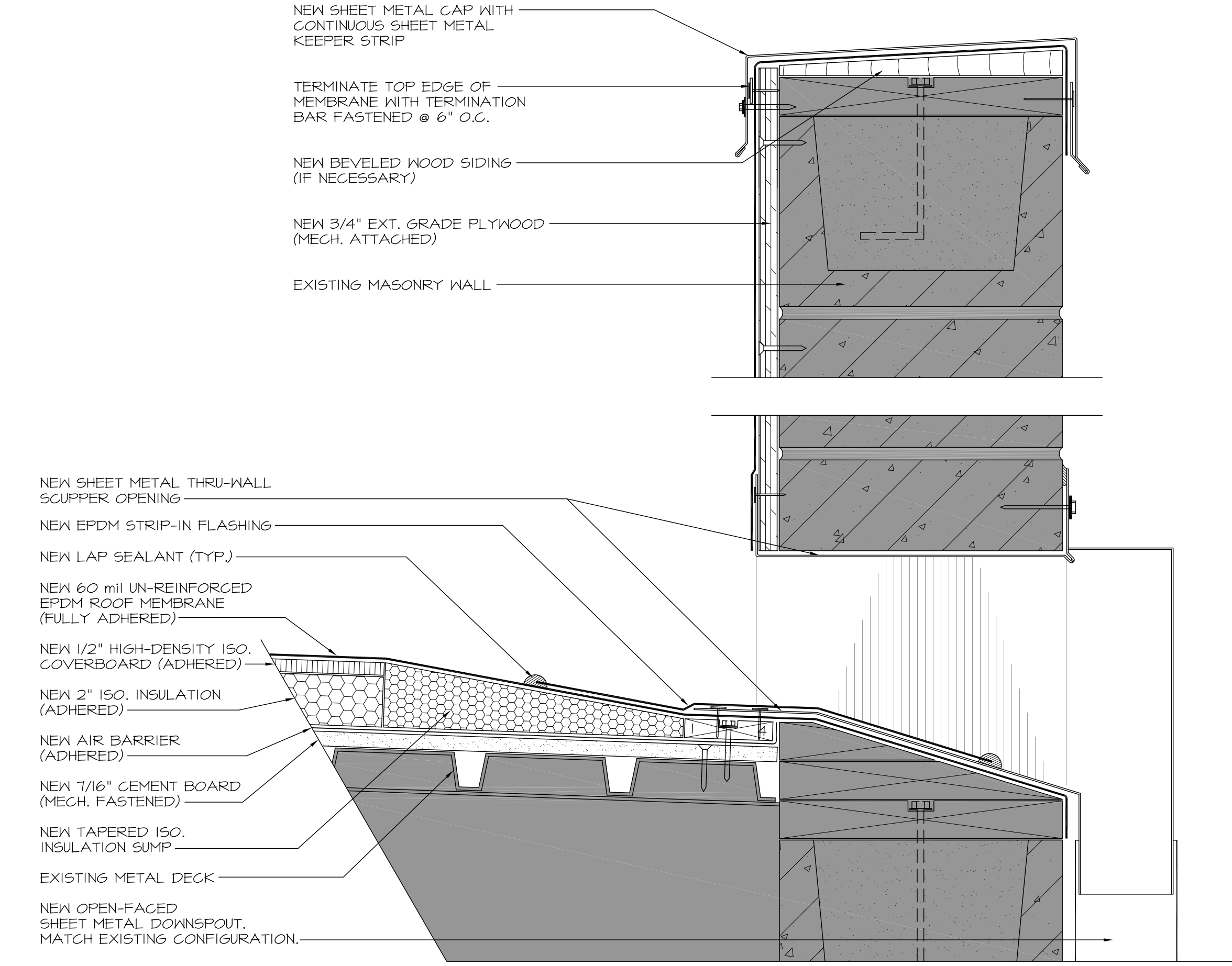
2 SCUPPER FLASHING DETAIL SCALE: 3/8"=1'-0"
