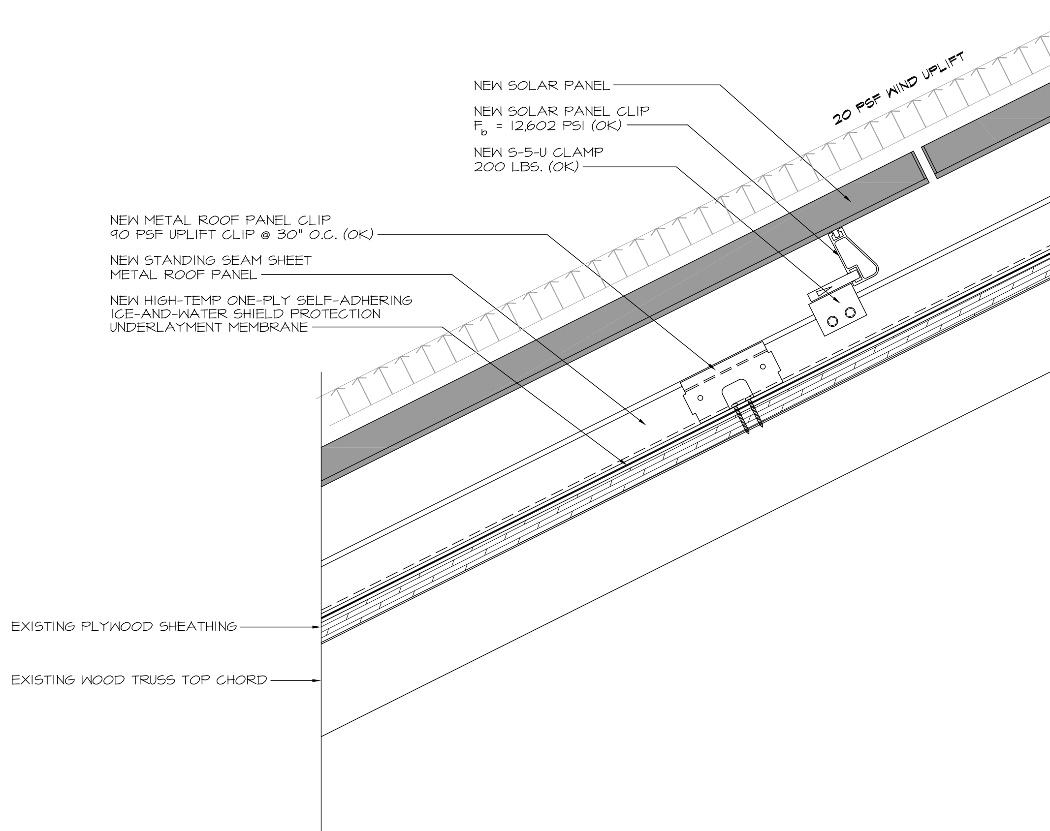
1 ROOF SYSTEM AND SOLAR PANEL SECTION - WIND ANALYSIS 2 SCALE: 3"=1'-0"
